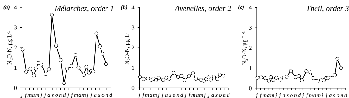
Fig. 3. Nitrous oxide concentrations between January 2007 and December 2008 in rivers at: (a) Mélarchez, first order; (b) Avenelles, second order and (c) Theil, third order.
