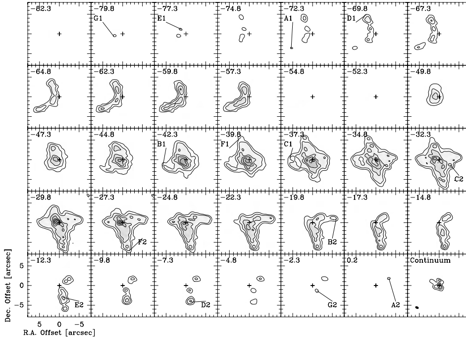
Fig. 1. Channel maps in the CO(2–1) line. The channel separation is 2.5 \text{ km s}^{-1} . The contours levels are 0.2, 0.5, and subsequent multiples of 0.5 Jy/beam. The coordinates of the map center are \alpha = 21^{\text{h}}02^{\text{m}}18^{\text{s}}.647 \delta = 36^{\circ}41'37''.8 (J2000.0) indicated by a cross. The synthesized beam ( 1''.07 \times 0''.85 ) is shown in the lower left corner of the continuum panel. The tips of the outflows are identified by letters A through G in the relevant panels, labelled by LSR velocity.
