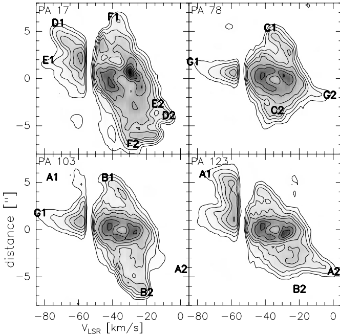
Fig. 3. Velocity-strip maps in the CO(2–1) line along the north-south bipolar outflow axis (P.A. 17^\circ ), and three east-west directions at P.A. of 78 , 103 , and 123^\circ (see Fig. 2). The contours are 0.25, 0.5, 0.75, 1 to 2.6 by 0.4 Jy/beam. The extremities of the outflows are indicated.
