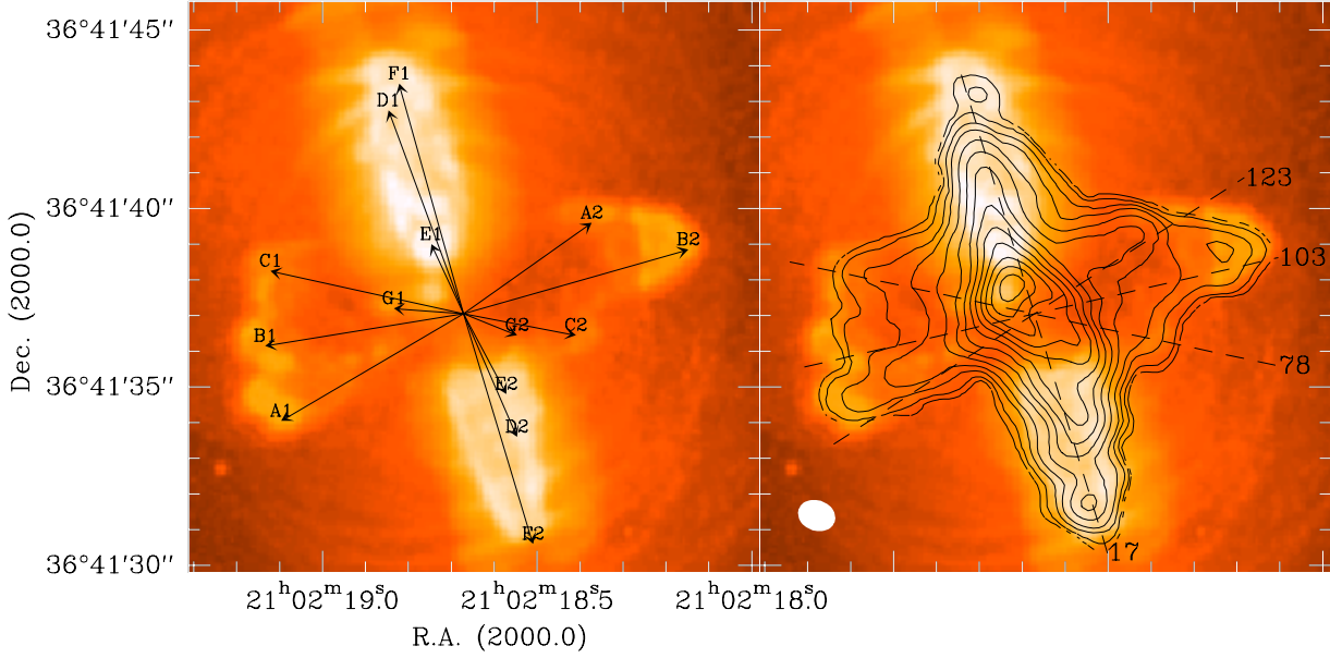
Fig. 2. The Plateau de Bure interferometer data compared to the \text{H}_2 1–0 S(1) line emission and nearby 2.15 \mu\text{m} continuum (in color) - from Sahai et al. (1998). The velocity integrated CO(2–1) emission is shown as contours (2, 4, 8, 12 to 72 by 6 Jy/beam) in the right panel, and the outflow axis are identified in the left panel (see also Fig. 1 and 3). The beam of the CO image is shown in the lower left corner of the right panel, with the locations of the position-velocity diagrams of Fig. 3
