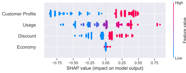
Figure 5: Summary Plot from SHAP, explaining a model trained excluding Visits .
