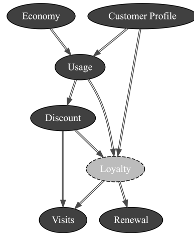
Figure 3: The causal Bayesian network used to generate the dataset. Loyalty is considered as a latent variable.
