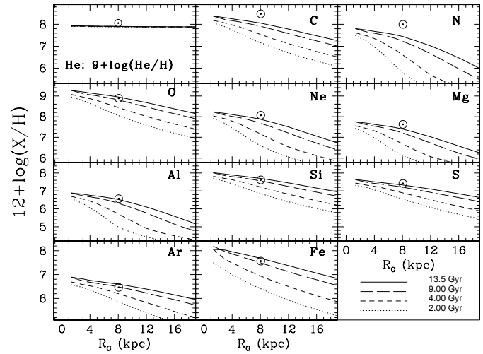
Fig. 4. Evolution of abundance profiles in the Milky Way disk, in the framework of the model presented in Sect. 2 and with the WW95 metallicity dependent yields. Curves show results at 2, 4, 9 and 13.5 Gyr, respectively (as indicated in the lower right panel). Because of the metallicity dependence of the yields, some elements (N, Al) have steeper abundance profiles than e.g. O, at all times. This is also the case for Fe, but the reason is its production mostly by SNIa. C and N are underproduced with respect to their solar system values, because yields from intermediate mass stars are neglected in this calculation. Metallicity dependent massive star yields from M92 considerably improve the situation concerning carbon (see Fig. 7), but not nitrogen. Solar abundances ( \odot ) were taken from Grevesse & Sauval (1998).
