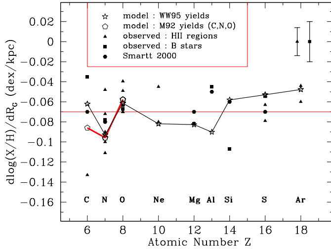
Fig. 8. Present day abundance gradients in the Milky Way disk: summary of models vs. observations. Model results are shown by open symbols (asterisks, for the WW95 yields, connected by a solid curve , and pentagons for the M92 yields, only for C, N and O). Observations (Table 1 for references) are shown by filled symbols . Notice the large discrepancy between the carbon gradients observed in B-stars and HII regions, respectively. An average gradient of -0.07 \pm 0.02 dex \text{kpc}^{-1} is compatible with most of the data and the model results. Most of the observed abundance gradients are rather well reproduced by the model, but the case of Al is problematic (see text).
