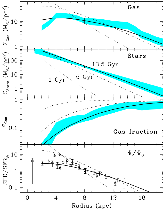
Fig. 3. Results of the chemical evolution model for the Milky Way disk and comparison to observations. In all panels, results are shown at three different epochs ( dotted curves : 1 Gyr, dashed curves : 5 Gyr, solid curves : 13.5 Gyr). The latter are to be compared to observations of present-day profiles in the Milky Way disk, shown as shaded regions in first three panels and within error bars in the lower panel. In all panels, the error bar at R_0 = 8 kpc indicates observed quantities in the solar neighborhood. References for data are given in BP99.
