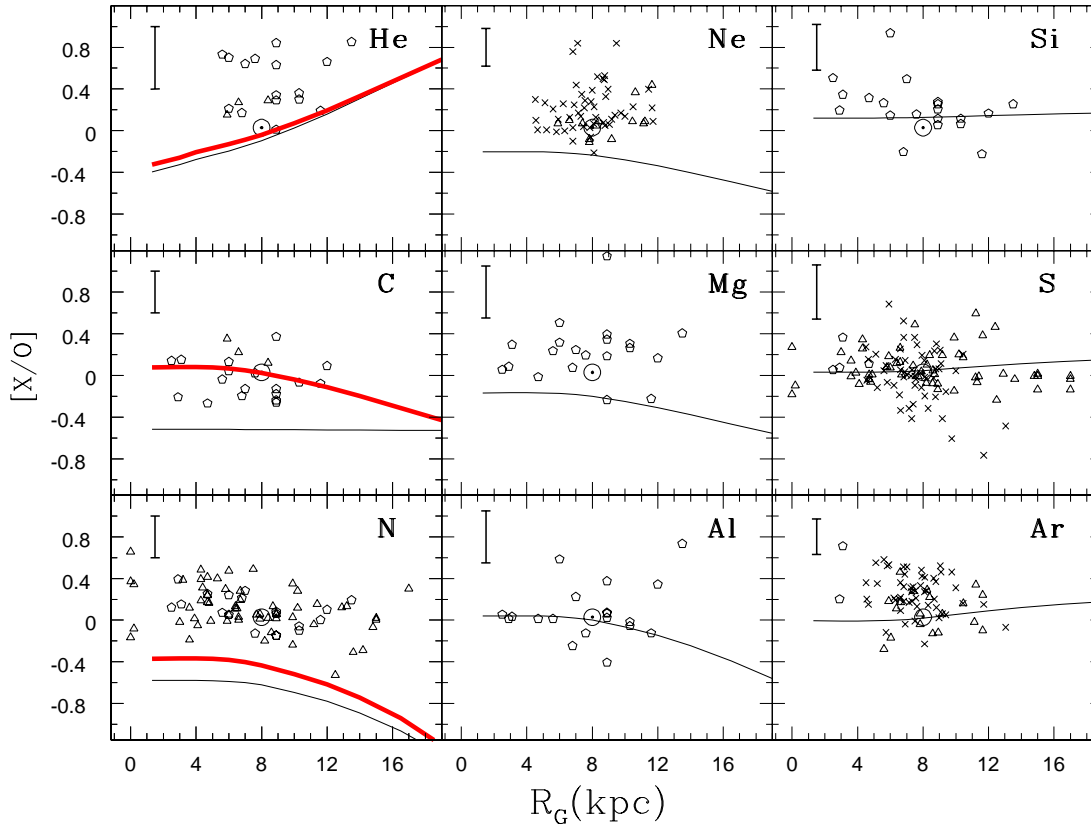
Fig. 9. Profiles of abundance ratios versus oxygen (normalised to the corresponding solar ratio: [X/O]=\log((X/O)/(X/O)_{\odot}) ) in the Milky Way disk. Observations are shown and compared to model results of this work. In all panels, the thin curves indicate results obtained with the WW95 yields, while the thick curves on the left side panels indicate results obtained with the M92 yields (leading to larger He/O, C/O and N/O abundance ratios). [Note: The flattening of theoretical profiles of abundance ratios in the inner disk is due to our use of yields for Z=Z_{\odot} even at metallicities larger than solar, because yields for such metallicities are not available in WW95 and M92]. Data (from references given in Table 1) concern HII regions ( triangles ), PNI ( crosses ) and B-stars ( pentagons ). The typical observational uncertainties for different element ratios are shown with error bars in the upper left corner of each panel. Notice that for Ne/O, the best values from type I PNs are given by the lower envelope of the data (see discussion in Sect. 4.3).
