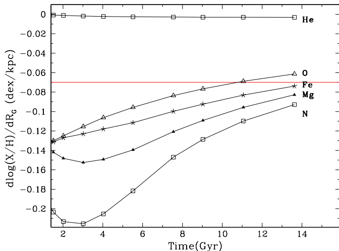
Fig. 5. Evolution of abundance gradients (expressed in dex/kpc) in the Milky Way disk (range: 4–14 kpc from the centre), in the framework of the model presented in Sect. 2 and with the WW95 metallicity dependent yields. Because of the inside-out formation scheme adopted here, gradients were steeper in the past. Because of the metallicity dependence of the yields of WW95, some elements, like N or Mg, have larger abundance gradients (in absolute value) than O. This is also the case for Fe, but the reason is its production mostly by SNIa.
