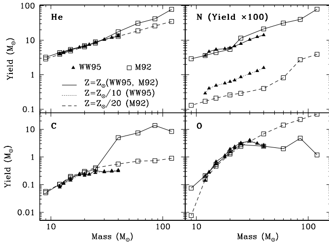
Fig. 2. Massive star yields of He, C, N and O for different initial metallicities, according to WW95 (filled triangles) and M92 (open squares); Solid curves: Z = Z_{\odot} , dotted curves: Z = 0.1 Z_{\odot} (for WW95), dashed curves: Z = 0.05 Z_{\odot} (for M92). There is good general agreement between the two calculations for stars with initial metallicity Z = Z_{\odot} . He, C and O are primary elements, i.e. their yields are independent of the initial stellar metallicity; the differences between the two sets of M92 yields for stars with M > 30 M_{\odot} are due to the metallicity dependent stellar winds. Nitrogen is produced as a secondary element in both WW95 and M92.
