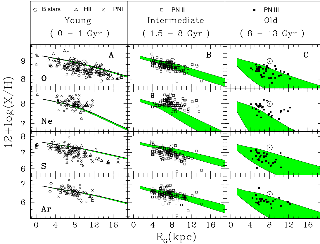
Fig. 10. Abundance profiles in the Milky Way disk at various epochs according to our model and comparison to objects of (hopefully) corresponding ages. From left to right, profiles are shown for young (Column A), intermediate (Column B) and old age (Column C) objects. In Case A belong B-stars, HII regions and planetary nebulae of type I; in Case B belong planetary nebulae of type II; and in Case C belong planetary nebulae of type III (see Sect. 4.4 for a discussion on ages). The corresponding model results are shown at time T = 12.5\text{--}13.5 Gyr or age = 0–1 Gyr (shaded area in A), T = 5.5\text{--}12 Gyr or age = 1.5–8 Gyr (shaded area in B) and T = 0.5\text{--}5.5 Gyr or age = 8–13 Gyr (shaded area in C). References for data are given in Table 1.
