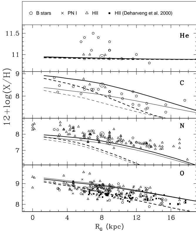
Fig. 7. Abundance profiles of He, C, N and O, at T = 9 Gyr ( dashed curves ) and T = 13.5 Gyr ( solid curves ), obtained with the WW95 yields ( thin curves , same as e.g. in Fig. 3), and the M92 yields ( thick curves ), in the framework of the model presented in Sect. 2. It can be seen that, compared to the WW95 yields, the M92 yields lead to considerably different results for C, to slightly different results for N, and to quasi-identical results for He and O. In particular, the M92 yields may explain completely the carbon abundance profile, with no need for any contribution from intermediate mass stars; on the contrary, nitrogen observations suggest that another source is mandatory.
