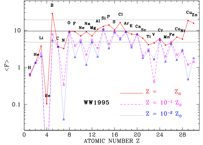
Fig. 1. Average overproduction factors (over a Kroupa et al. (1993) IMF, see Eq. 4) of the yields of Woosley & Weaver (1995) for 3 different initial stellar metallicities, covering reasonably well the metallicity evolution of the Milky Way disk. The solid horizontal line is placed at F_{\text{oxygen}} and the two dotted horizontal lines at half and twice that value, respectively. Most of the intermediate mass elements are nicely co-produced (within a factor of two). The “odd-even effect” is clearly seen (e.g. in the cases of Na, Al, P, etc.); notice the small (but significant) metallicity dependence of the Ne and Mg yields. N behaves as a pure “secondary” element. The elements He, C, N, Li and Be obviously require another production site.
