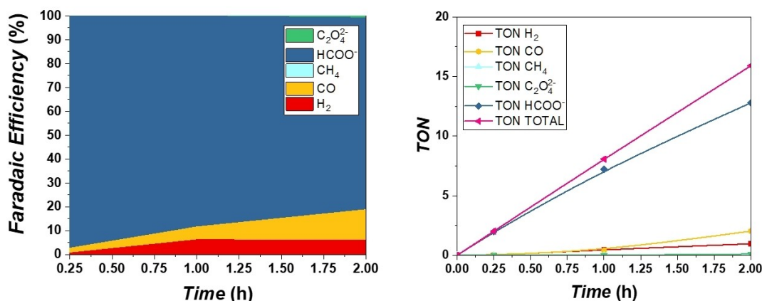
Figure 5. Faradaic efficiency (FE, left) and TON (right) for the CO 2 reduction products and hydrogen evolved during 2 h CPE experiments run at −2.43 V vs Fc + /0 , in the presence of 0.5 mM solutions of Ir OPyr in DMF 0.1 M nBu 4 NPF 6 containing 4.6 M H 2 O under CO 2 -saturated atmosphere (Hg working electrode).
