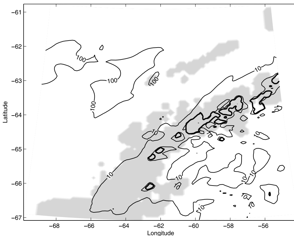
Figure 10. Map of the minimum Richardson number in the altitude range 12–20 km, from domain 2 on 7 October 2005, 0900 UT. The thick contour outlines regions of static instability ( Ri < 0 ). Other contour lines indicate Ri values of 1, 10 (labeled), and 100 (labeled).
