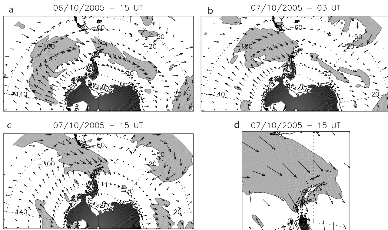
Figure 4. (a–c) Horizontal winds from 3-h forecasts of the ECMWF operational model on the 850-hPa surface. Hours are indicated above each plot. Grey shading corresponds to areas where the modulus of the horizontal wind is greater than 20 \text{ m s}^{-1} . Regions where the 850-hPa isobar is below the surface are shaded in black. (d) A close-up of the Antarctic Peninsula from Figure 4c.
