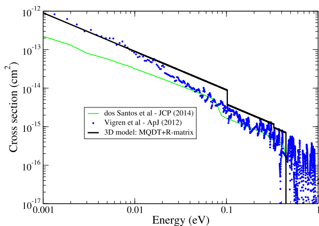
Fig. 5 DR of N_2H^+ at low energy of the incident electron within the 3D model. Blue symbols: CRYRING measurements [13]. Green line: Results obtained with the complex Kohn variational method combined with the normal mode approximation [23]. Black line: Present results relying on R-Matrix-normal mode approximation combined with MQDT frame transformation
