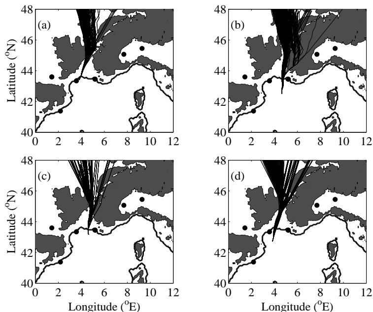
Fig. 12. Back trajectories ending at 3.9^{\circ}\text{E}/43.4^{\circ}\text{N} (way-point A) (a) , 4.65^{\circ}\text{E}/42.5^{\circ}\text{N} (way-point F) (b) , 4.7^{\circ}\text{E}/43.2^{\circ}\text{N} (way-point C) (c) and 3.88^{\circ}\text{E}/42.75^{\circ}\text{N} (way-point E) (d) . The back trajectories ending points correspond to the starting and ending points of the ARAT legs and the aerosol plumes detected by the lidar LEANDRE-2 on board the ARAT. The altitude of the ending points is 50 m. The ending times of the back trajectories are 16:00 and 17:00 UTC for the first and second row, respectively. Filled black dots indicate the cities of Barcelona, Toulouse, Montpellier, Marseille/Fos-Berre, Lyon, Torino and Milano.
