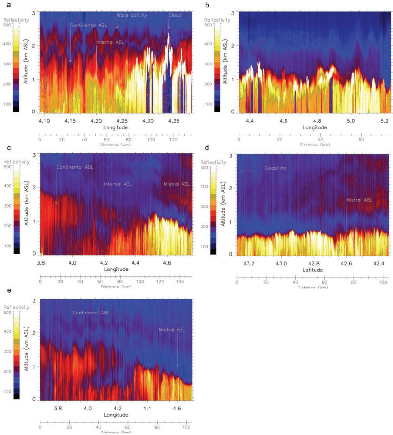
Figure 14. Atmospheric reflectivity at 0.73\ \mu\text{m} as obtained from LEANDRE 2 along (a) leg AD and (b) leg DE of the morning flight and along (c) leg AF, (d) leg FC, and (e) leg CE of the afternoon flight. Way points A and D are to the left of Figures 14a and 14b, respectively. Way points A, C, and E are to the left of Figures 14c, 14d, and 14e, respectively.
