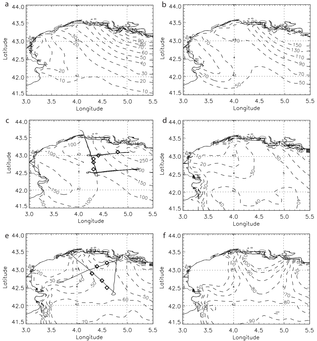
Figure 8. Surface sensible heat fluxes over the Mediterranean forecasted on 24 March 1998 by the French operational forecast model ALADIN at (a) 0600, (b) 0900, (c) 1200, (d) 1500, (e) 1800, and (f) 2100 UTC. Units are \text{W m}^{-2} . Superimposed are the ARAT tracks during F02 and F03 (solid lines). Diamonds indicate the positions where averaged turbulent heat fluxes were computed at the lowest level flown by the aircraft.
