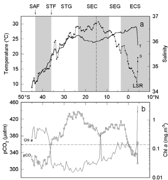
Figure 7. Distribution of (a) surface salinity and temperature ( ^{\circ}\text{C} ) and (b) surface \text{pCO}_2 ( \mu\text{atm} ) and chlorophyll a ( \text{mg m}^{-3} ) along the line A14. ECS is Equatorial Current System, SEG is South Equatorial Gyre, SEC is South Equatorial Current, STG is Subtropical Gyre, STF is Subtropical Front, SAZ is Subantarctic zone, and SAF is Subantarctic Front. Vertical dashed line in Figure 7a represents subtropical/subequatorial transition. Horizontal dashed line represents the mole fraction in dry air ( x\text{CO}_2 ) for 1995 (359 ppm) according to Keeling et al. [1995].
