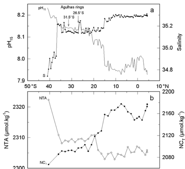
Figure 9. Meridional evolution of (a) salinity and \text{pH}_{15} and (b) \text{NC}_T and NTA in \mu\text{mol kg}^{-1} along the SACW 13 ^{\circ}\text{C} isotherm.
