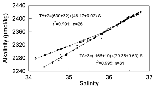
Figure 8. Relationship between total alkalinity ( \mu\text{mol kg}^{-1} ) and salinity in surface waters along line A14. The corresponding linear regressions are reported.
