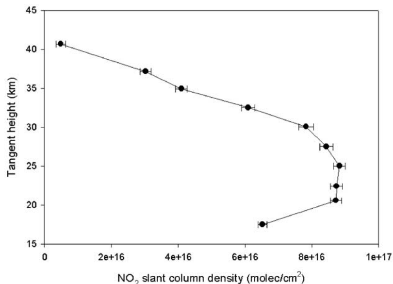
Figure 7. Measured SCD profile (see Figure 6 for details of geo-location).
