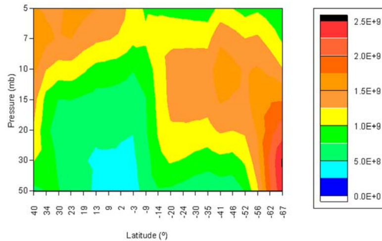
Figure 10b. CMAM contour plot of NO 2 number density ( \text{cm}^{-3} ) over same latitude range and solar conditions: October average.
