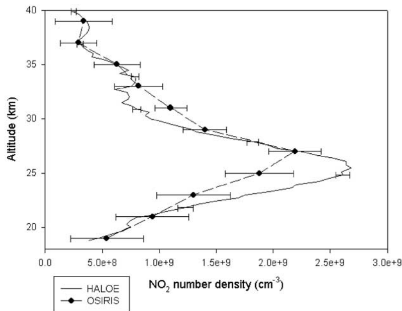
Figure 12d. Mid-latitude winter (28.02.2002) sunset coincidence between HALOE and OSIRIS (lat = 59.7^\circ ).
