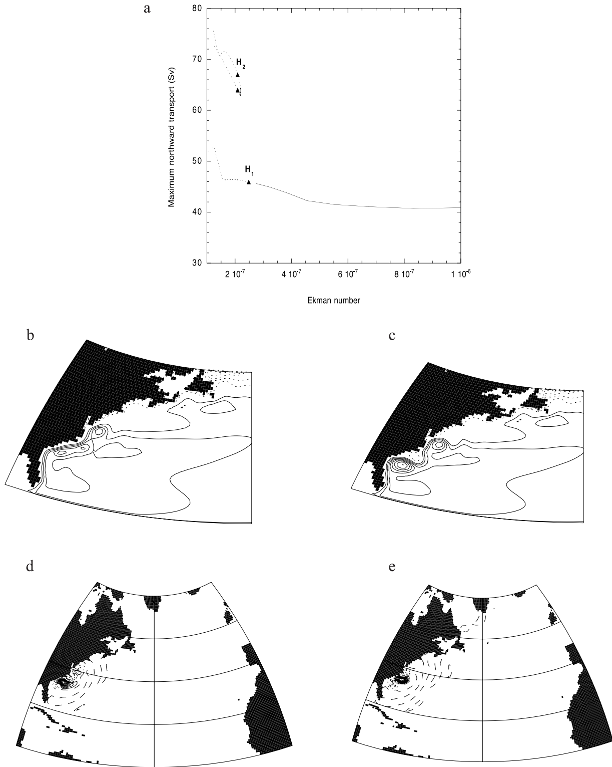
Figure 6. (a) Bifurcation diagram for a barotropic shallow water model of the North Atlantic with the Ekman number as control parameter. The nondimensional Ekman number, E = A_H / (2\Omega r_0^2) , where \Omega and r_0 are the angular frequency and radius of the Earth, respectively, is plotted on the abscissa, while the maximum northward volume transport is plotted on the ordinate. Solid (dotted) branches indicate stable (unstable) steady states, as usual, whereas the Hopf bifurcation points are indicated by triangles. (b and c) Contour plots of the layer thickness anomaly for two coexisting unstable solutions at E = 1.6 \times 10^{-7} . The contour levels are scaled with respect to the maximum value of the field; only a small part of the domain, ( 85^\circ\text{W} – 45^\circ\text{W} , 24^\circ\text{N} – 51^\circ\text{N} ), is shown: “deflected” (Figure 5b) and “separated” Gulf Stream (Figure 5c). (d and e) Spatial pattern of the linear oscillatory mode at H_1 in Figure 6a. Layer thickness anomalies for the real (Figure 6d) and imaginary part (Figure 6e) are shown. From Schmeits and Dijkstra [2000].
