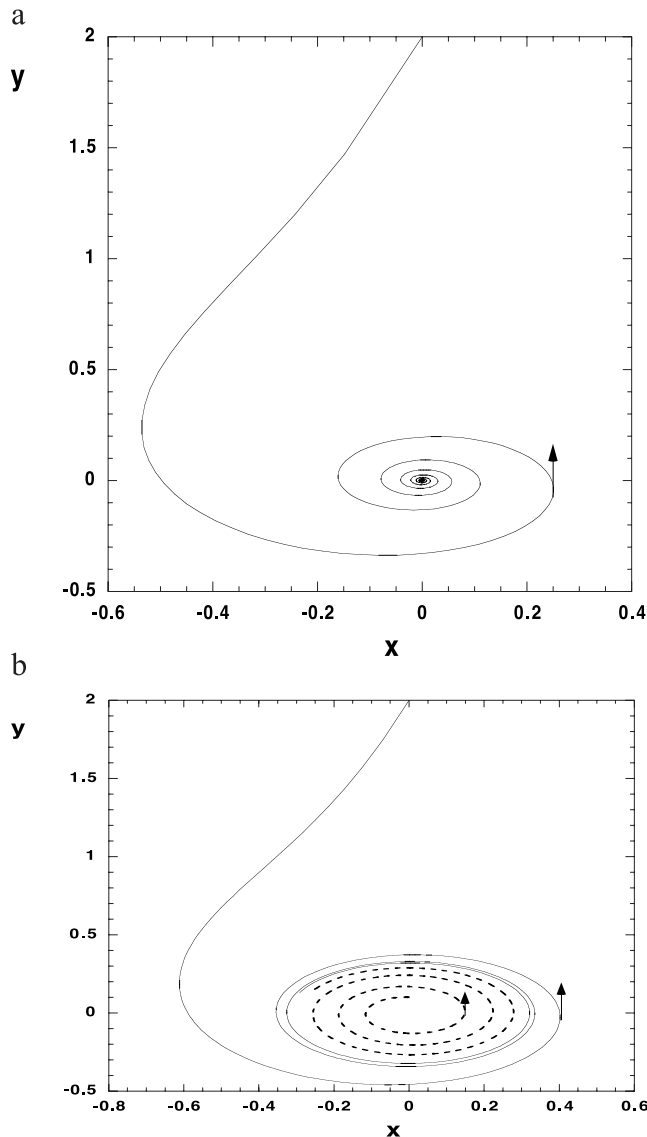
Figure B2. Trajectories of the reduced equations (B4) for the Hopf bifurcation: (a) before the bifurcation at \lambda = 0 ( \lambda = -0.1 ) and (b) after the bifurcation ( \lambda = 0.1 ). The secondary parameter value is \omega = 1.0 , and both graphs show a trajectory that starts at the point (0, 2) . In Figure B2b an additional trajectory starting at (0, 0.1) is shown as the dashed curve. Arrows indicate the tangent at that point in the direction of evolution along the given curve.
