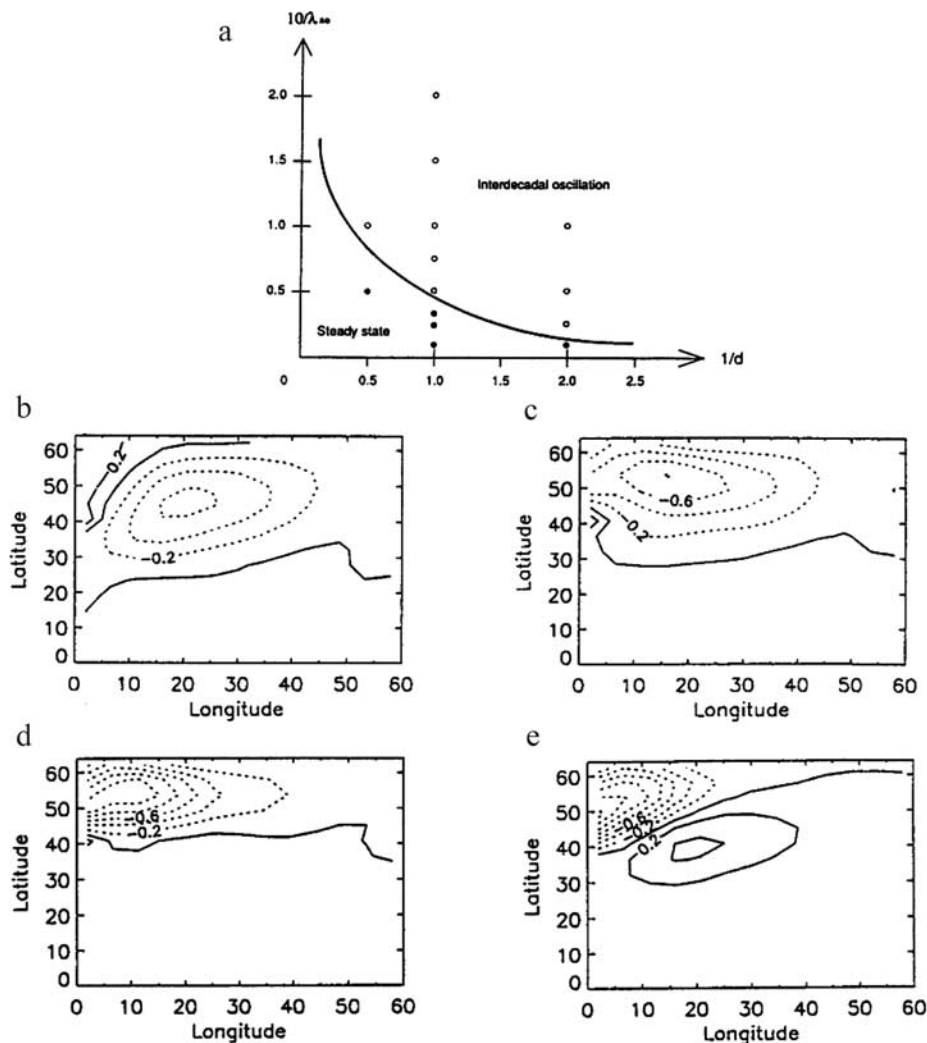
Figure 15. (a) Regime diagram for a hybrid coupled model. The parameters d and \lambda_{oa} are the atmospheric EBM's thermal diffusivity and the proportionality constant for the air-sea heat flux, respectively. Solid circles in both diagrams indicate numerically computed steady states; open circles indicate periodic solutions. From Chen and Ghil [1996]. (b–e) Interdecadal oscillation in the hybrid coupled model. SST anomaly patterns are shown at intervals of about 5.5 years to cover roughly half the period of the 44-year oscillation.
