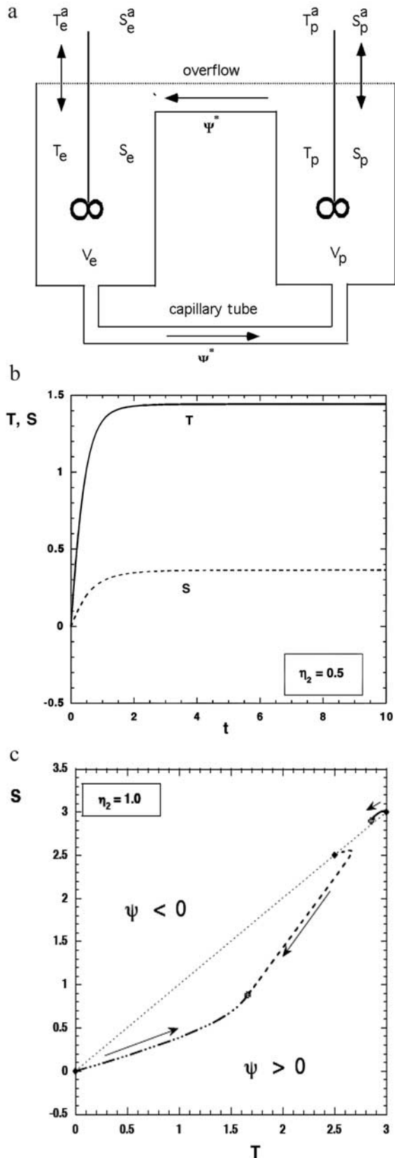
Figure 10. (a) Sketch of the two-box model setup of Stommel [1961]. Two reservoirs contain well-mixed water and are connected through an overflow and a capillary tube. The circulation is driven by density gradients between the boxes; these are due to heat and salinity fluxes at the surface. The direction of flow between boxes corresponds to a thermally dominated solution, with \Psi > 0 and implied sinking in the polar and rising in the equatorial box. (b) Evolution of T(t) and S(t) for a solution with zero initial data, T(0) = S(0) = 0 , \eta_1 = 3.0 , \eta_2 = 0.5 , and \eta_3 = 0.3 . (c) Trajectories in the (T, S) plane for three different initial states (shown by diamonds) that can lead to two different steady states (shown by crosses). Here \eta_2 = 1.0 , while \eta_1 = 3.0 and \eta_3 = 0.3 , as in Figure 10b.
