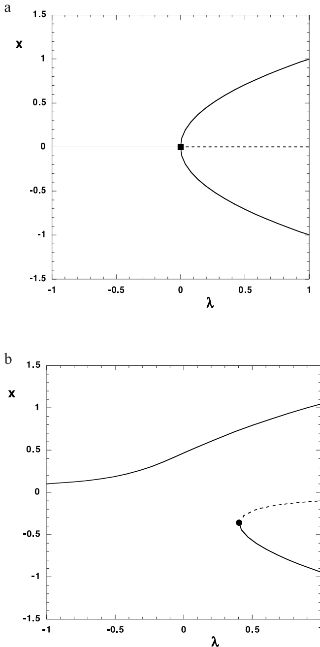
Figure B1. (a) Bifurcation diagram of the pitchfork bifurcation in the system f(x, \lambda) = \lambda x - x^3 . (b) Perturbed pitchfork bifurcation diagrams for the system f(x, \lambda) = \epsilon + \lambda x - x^3 for \epsilon = 0.1 . Solid lines indicate stable solutions, and dashed lines indicate unstable ones. The bifurcation points are marked by a circle and square.
