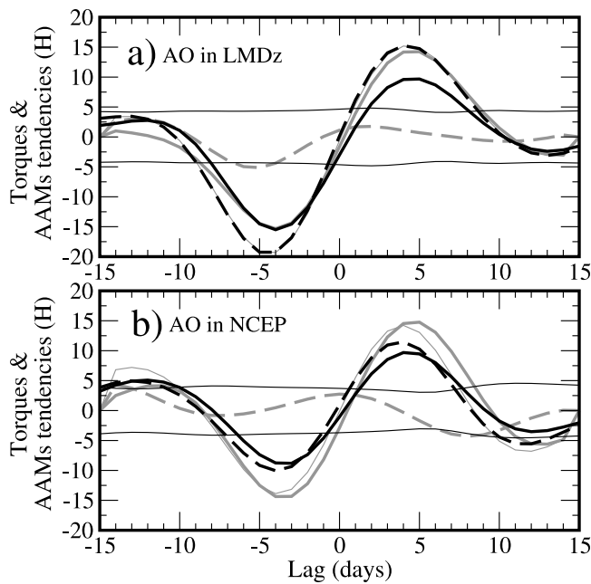
Figure 7. Composites of different terms in the AAM budget, keyed to minus the IS AO: (a) LMDz model and (b) NCEP reanalysis. IS M_{\Omega} tendency (thick grey solid lines), IS M_R tendency (thick grey dashed lines), IS total AAM ( M ) tendency (thin grey lines), IS T_M (thick black solid lines), and IS total torque T (thick black dashed lines). The thin black lines are 1% confidence levels for the IS T_M , evaluated with a Student test with N degrees of freedom, N being the number of dates selected to build the composites.
