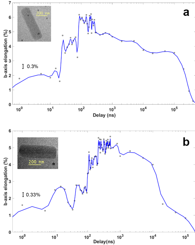
Figure 1. Time-resolved length measurements of two SCO particles with length of 600 nm. The excitation laser wavelength was 532 nm. (a) Particle 1; the laser power on the specimen was 4 \mu\text{J}/\text{cm}^2 . (b) Particle 2; the laser power on the specimen was 3.5 \mu\text{J}/\text{cm}^2 . TEM images of the respective particles are shown in the insets. The error bar of all measurements is shown on the left.
