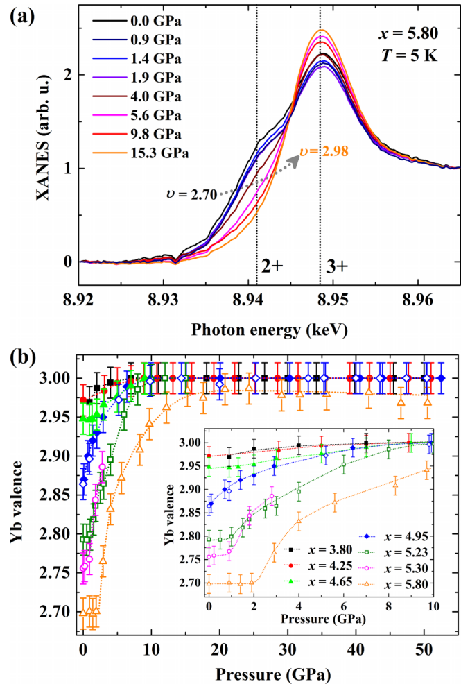
FIG. 2. (a) Yb L_3 XANES spectra of \text{YbMn}_6\text{Ge}_{0.2}\text{Sn}_{5.8} at 5 K for different applied pressures. (b) Pressure dependence of the Yb valence at 5 K of \text{YbMn}_6\text{Ge}_{6-x}\text{Sn}_x extracted from the XANES spectra. The inset shows an enlargement of the low-pressure region ( P < 10 GPa). Room-temperature data are also shown for x = 4.95 (open blue diamonds).
