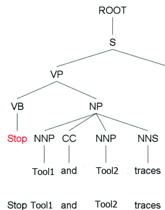
Figure 6: Syntax tree for Stop instructions
