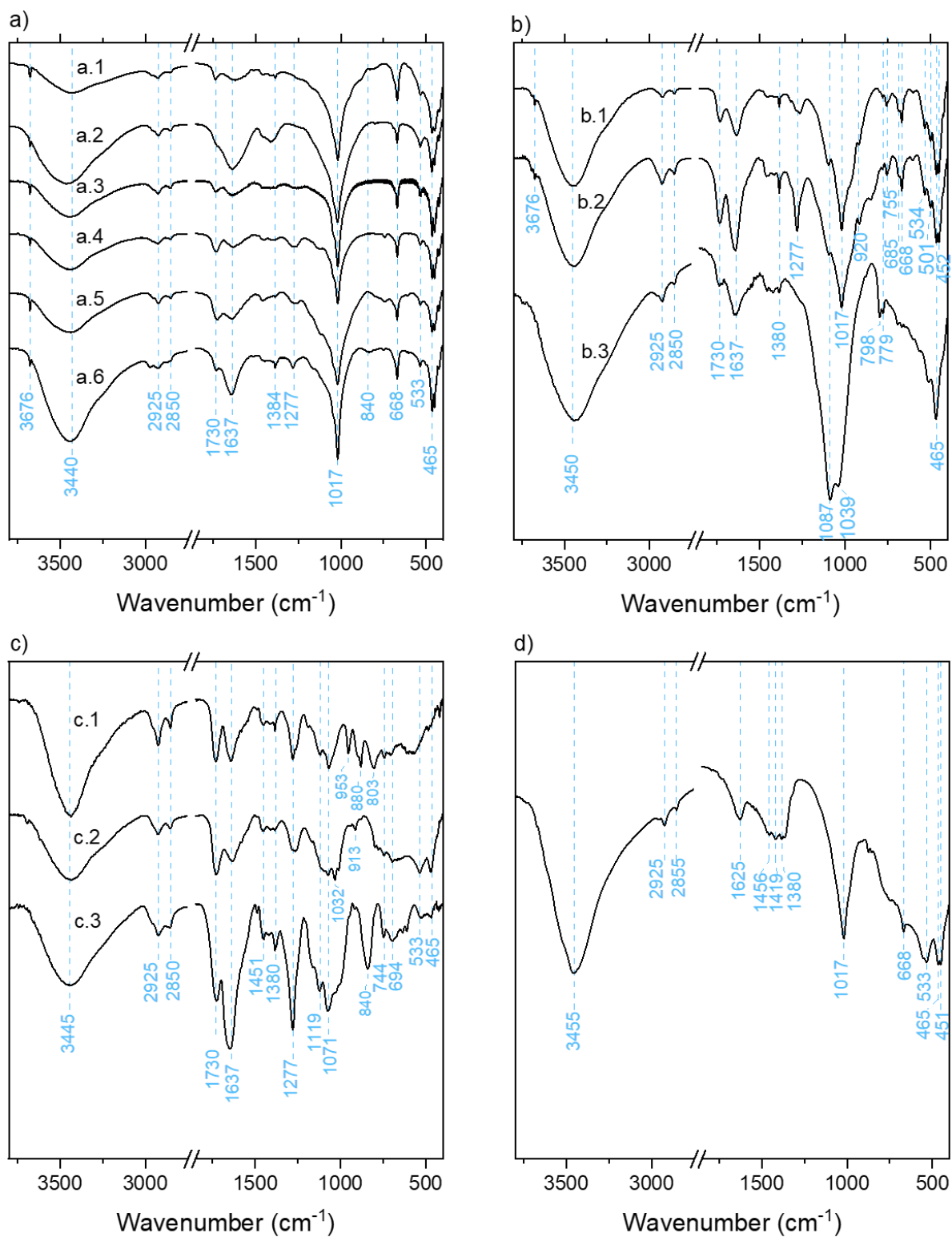
Figure 3. FTIR transmission spectra (arbitrary units on the Y-axis) of paint of a) German aircraft: a.1 JU88 ; a.2 HE111 – primer ; a.3 HE111 – layer 2 ; a.4 HE111 – layer 4 ; a.5 DO217 ; a.6 HE177 ; b) American aircraft: b.1 LOP38 – layer 3 ; b.2 LOP38 – layer 2 ; b.3 RAP47D ; c) French aircraft: c.1 DE520 ; c.2 LA298 ; c.3 MS733 and d) Italian aircraft: MAMC202.
