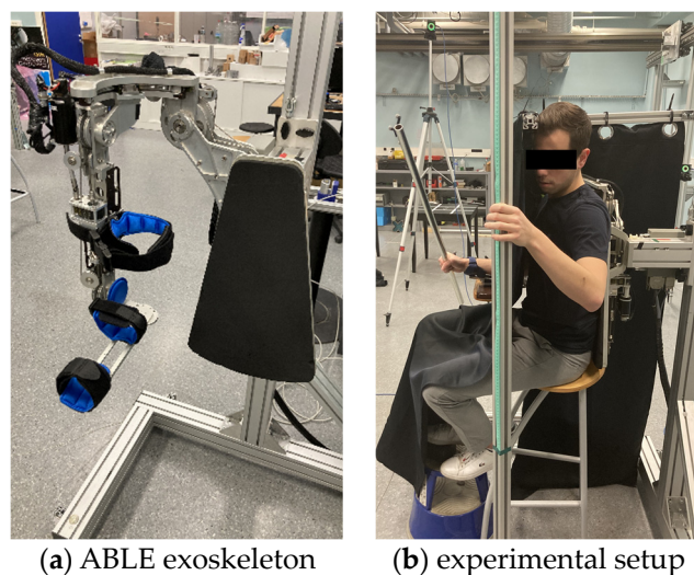
Figure 1. (a) The ABLE exoskeleton comprising three rotational axes at the shoulder and one at the level of the elbow. Foam and Velcro fixations are used to secure the forearm and upper arm of the user to the structure. (b) A participant manipulates a bar with his right hand during an experimental trial. Perceived partial length was indicated using an adjustable marker on a vertical pole positioned to the left of the participant.
