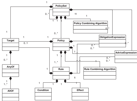
Figure 1. The XACMLv3 policy language mode [11]
