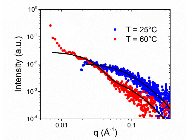
Figure 13. Small-angle X-ray scattering (SAXS) patterns recorded for 1 wt.% aqueous dispersion of \text{PN}_{5k}\text{-}b\text{-PD}_{5k} at 25 and 60 °C (pH = 4).
