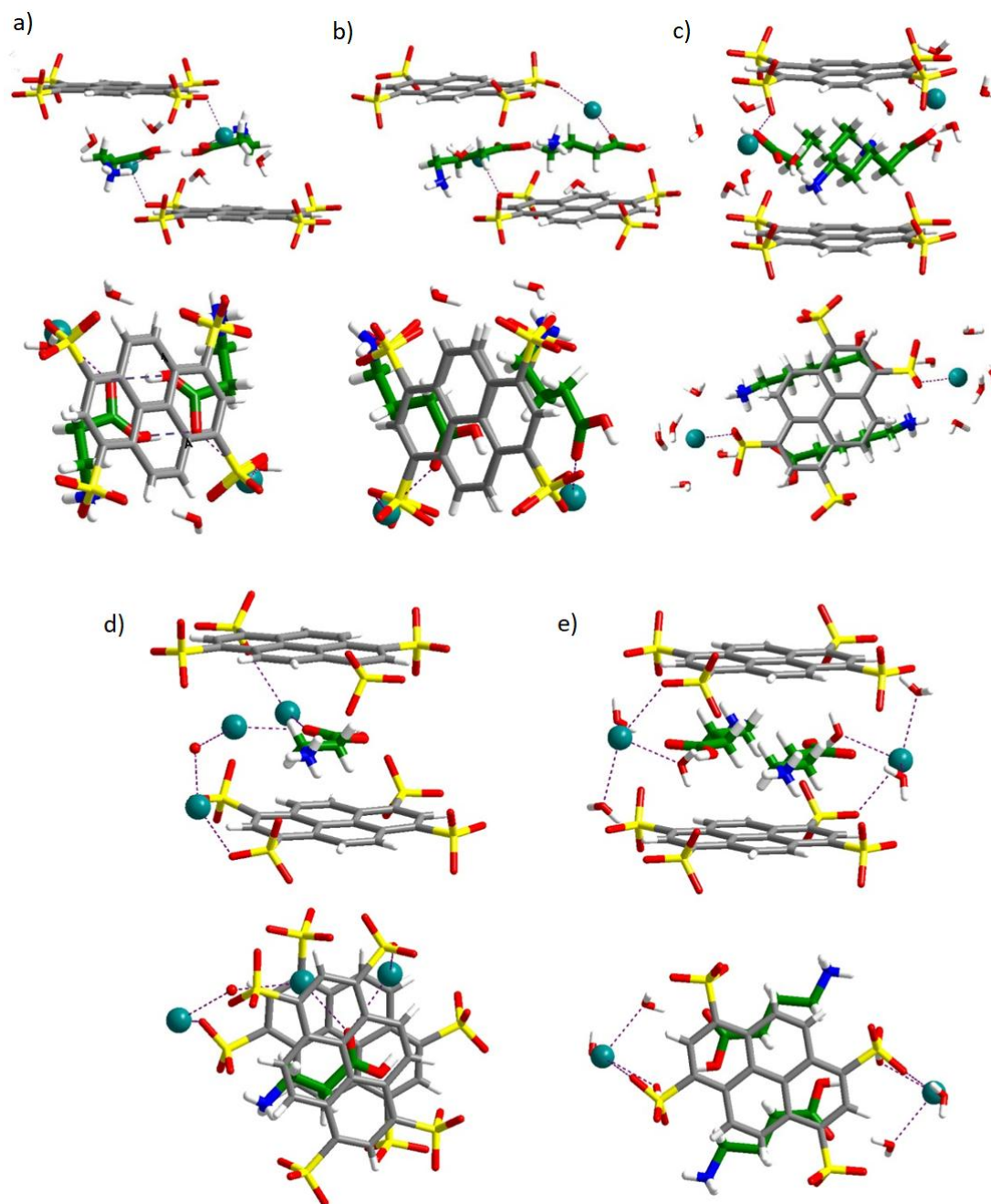
Figure 5. Side and top views of X-ray co-crystal structures for (a) [PTNaC2], (b) [PTNaC3] (c) [PTNa+4] (d) [PT++C2], (e) [PTSKC3] [Colors for elements: red, oxygen; yellow, sulfur; blue, nitrogen; grey, carbon; white, hydrogen; teal, metal cation; green, carbons of guests]
