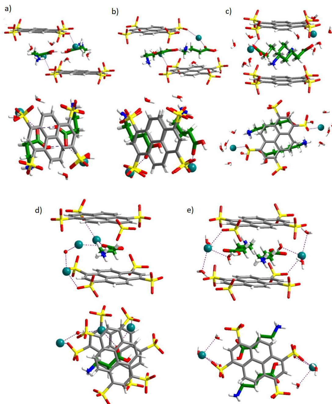
Figure 5. Side and top views of X-ray co-crystal structures for (a) [PTNaC2], (b) [PTNaC3] (c) [PTNaC4] (d) [PTSCC2], (e) [PTSKC3] [Colors for elements: red, oxygen; yellow, sulfur; blue, nitrogen; grey, carbon; white, hydrogen; teal, metal cation; green, carbons of guests]
