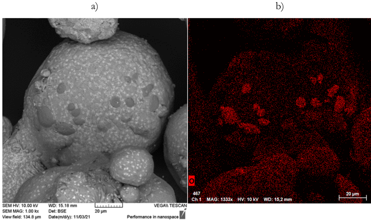
Fig. 14. (a) SEM pictures of thermally affected powder and (b) EDS analysis of oxygen.
