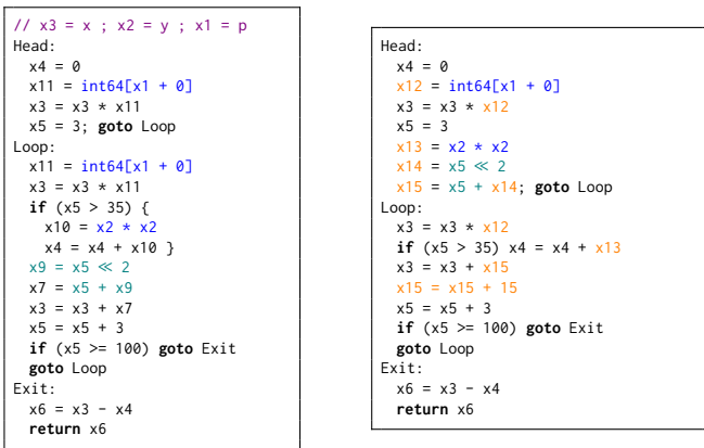
Figure 4: Unrolled (left) and optimized (right) RTL code
