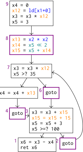
Figure 5: Optimized BTL
