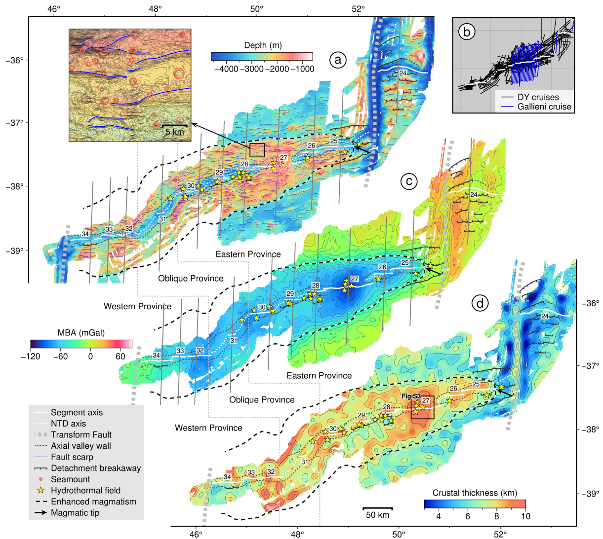
Figure 2. Geological mapping and gravity inversion. (a) Geological interpretation superimposed on the bathymetry map (see legend for symbols). Cross-axis profiles are shown in Figure 3. The inset shows examples of picking seamounts and faults. (b) Gravity survey tracks of the DY cruises (black lines) and the Gallieni cruise (blue lines). (c) MBA map calculated by subtracting the predicted gravity effect based on shipboard bathymetry and a 6 km-thick model crust from the FAA in Figure S2b. The grid spacing of the FAA and MBA maps is 0.5 min. (d) Crustal thickness, calibrating the center of segment #27 (50.5°E) to 9.5 km, which is defined by depths to the Moho interfaces (Jian et al., 2017; Li et al., 2015). Black square shows the location in Figure 7.
