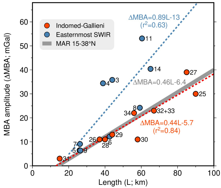
Figure 9. Along-axis MBA amplitude ( \Delta MBA ) as a function of segment length ( L ). Data included are the Indomed-Gallieni (red circles and red dashed fitting line by this study), the easternmost SWIR (blue circles and blue dashed fitting line) (Cannat et al., 1999), and the slow spreading MAR 15-38°N (thick gray fitting line) (Detrick et al., 1995; Lin et al., 1990; Thibaud et al., 1998).
