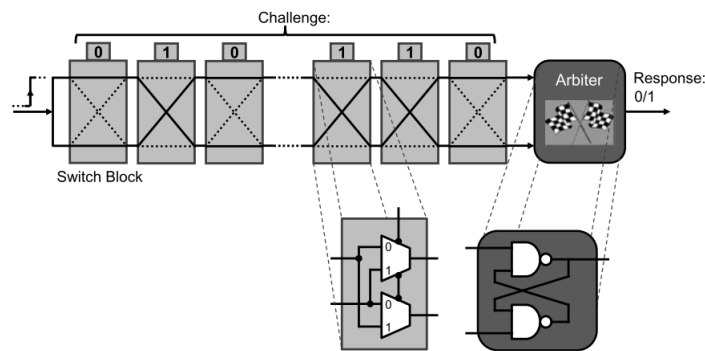
Fig. 3 The Structure of the Arbiter PUF.
