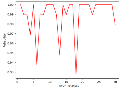
Fig. 11 APUF Reliability.
