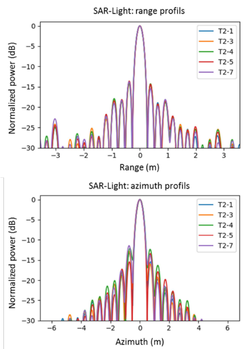
Fig. 5. Impulse responses measured over 5 trihedrals.
