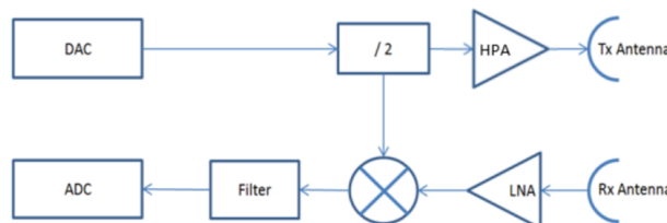
Fig. 2. FMCW Radar block diagram.
