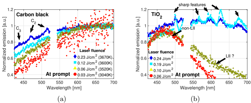
Fig. 7: Effect of laser fluence F on laser-induced emission spectra at prompt for (a) carbon black and (b) TiO 2 nanoparticles. The temperature inside the legend for carbon black particles is obtained from the spectrum fitting of the Planck function. Spectra are normalized by the value at 650 nm, except for the case of TiO 2 F = 0.06 J/cm 2 and F = 0.10 J/cm 2 , which are normalized by max value at 470 nm for visualization purpose.
