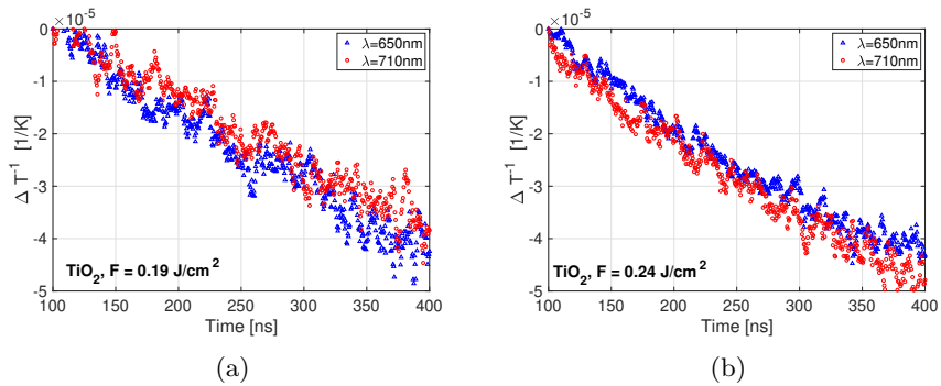
Fig. 16: Time evolution of \Delta T^{-1} of pure TiO 2 nanoparticles LIE for two laser fluences at (a) F=0.19 and (b) F=0.24 \text{ J/cm}^2 .
