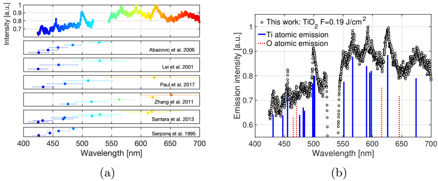
Fig. 9: Normalized emission spectra of TiO 2 for F = 0.19 \text{ J/cm}^2 with (a) gaussian fit of band emission of LIF from literature [15, 20, 72, 73, 75, 76] and (b) Ti and O atomic emissions from NIST [77] corresponding to peak location of emission spectra. The intensities of each transition are adapted for a clear view with the curve, not expressing the relative intensities.
