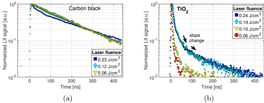
Fig. 11: Temporal evolution of laser-induced emission of (a) carbon black and (b) TiO 2 nanoparticles at 450 \pm 10 nm detection wavelength. Each profile is normalized by its maximum value.
