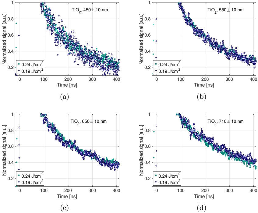
Fig. 13: Normalized temporal evolution of high-purity TiO 2 nanoparticles at different laser fluences at detection wavelengths of (a) 450 \pm 10 , (b) 550 \pm 10 , (c) 650 \pm 10 and (d) 710 \pm 10 nm. All profiles are normalized with the value of the signal at 100 ns.
