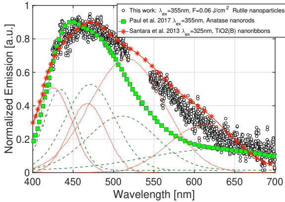
Fig. 8: Emission spectra of TiO 2 nanoparticles at prompt under laser fluence F = 0.06 \text{ J/cm}^2 (black round points). The LIF emission spectra (square and star symbol) are from gaussian fitted spectra (green dashed line from Paul et al. [72], red dotted lines from Santara et al. [73]).
