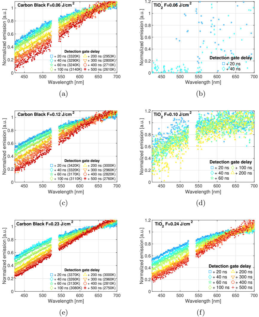
Fig. 10: Effect of gate delay (gate width = 20 ns) on emission spectra of laser-induced emissions of (a,c,e) carbon black nanoparticles and (b,d,f) rutile \text{TiO}_2 nanoparticles. The temperature given inside the legend for carbon black particles is obtained from spectrum fitting. Spectra are normalized with the value of the spectrum at 650 nm.
