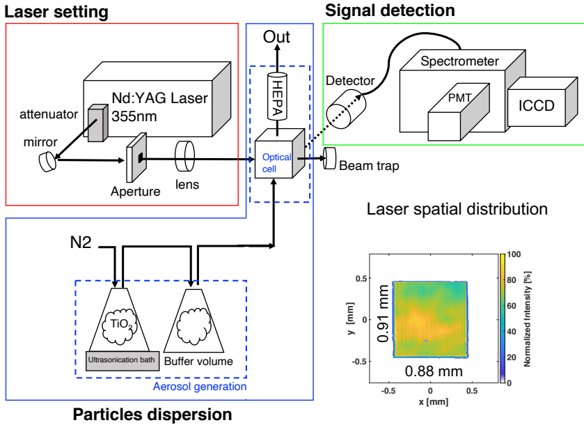
Fig. 5: Schematic presentation of the experimental set-up developed to investigate laser-induced emission from TiO 2 nanoparticle-laden aerosol using a pulse YAG laser at 355 nm with a nearly top-hat spatial profile (bottom-right).
