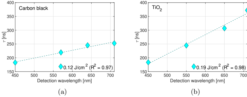
Fig. 14: Decay characteristic times of LIE signal for (a) carbon black and (b) TiO 2 as a function of detection wavelength. The R^2 value inside the legend represents the coefficient of determination for the fitting procedure. The dotted lines are the results of the linear fitting.
