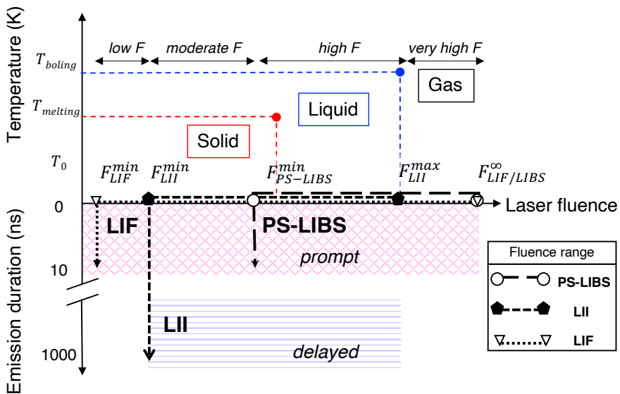
Fig. 4: Schematic presentation of the particle phase information related to the temperature (top) and to the LIE characteristic emission signals (bottom) as a function of the typical fluence range of different LIE signals.
