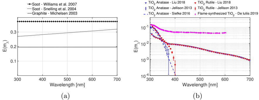
Fig. 1: Absorption function E(m_\lambda) of (a) carbonaceous particles [46, 49, 55] and (b) TiO 2 nanoparticles (in log scale) [51–54].
