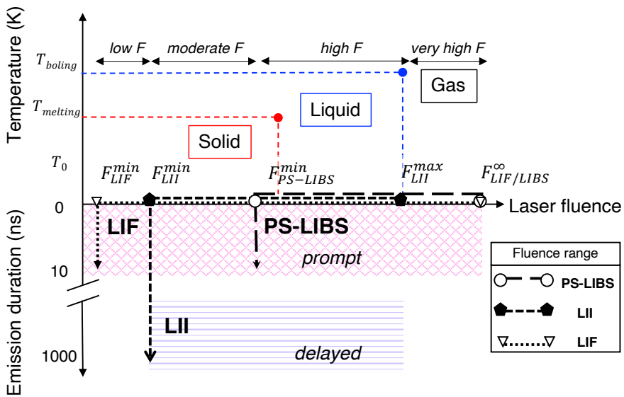
Fig. 4: Schematic presentation of the particle phase information related to the temperature (top) and to the LIE characteristic emission durations (bottom) as a function of the typical fluence range of different LIE signals.
