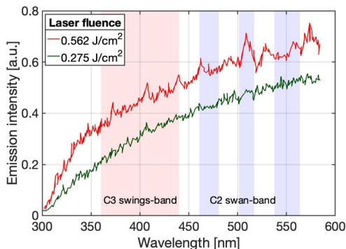
Fig. 3: Laser-induced light emission under different laser fluences at HAB = 2 cm in flame spray synthesis of TiO 2 nanoparticles at prompt detection timing obtained in [42]. C 2 and C 3 bands from [61] are indicated in blue and red, respectively.
