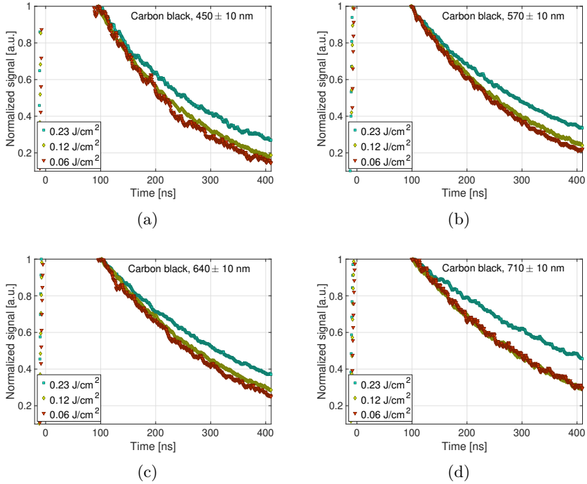
Fig. 12: Normalized temporal evolution of carbon black nanoparticles at different laser fluences at detection wavelengths of (a) 450 \pm 10 nm, (b) 570 \pm 10 nm, (c) 640 \pm 10 nm and (d) 710 \pm 10 nm. All profiles are normalized with the value of the signal at 100 ns.
