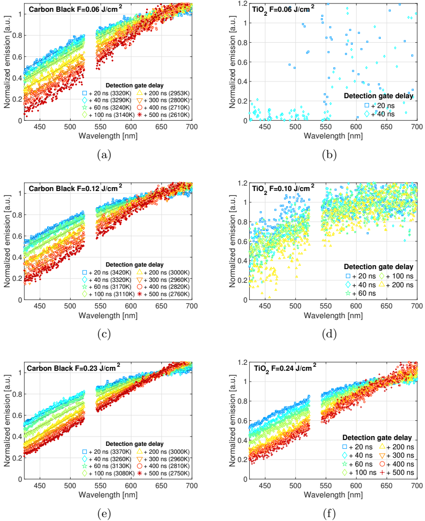
Fig. 10: Effect of gate delay (gate width = 20 ns) on emission spectra of laser-induced emissions of (a,c,e) carbon black nanoparticles and (b,d,f) rutile TiO 2 nanoparticles. The temperature given inside the legend for carbon black particles is obtained from spectrum fitting. Spectra are normalized with the value of the spectrum at 650 nm.
