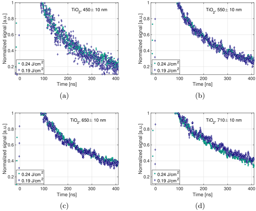
Fig. 13: Normalized temporal evolution of high-purity TiO 2 nanoparticles at different laser fluences at detection wavelengths of (a) 450 ± 10, (b) 550 ± 10, (c) 650 ± 10 and (d) 710 ± 10 nm. All profiles are normalized with the value of the signal at 100 ns.
