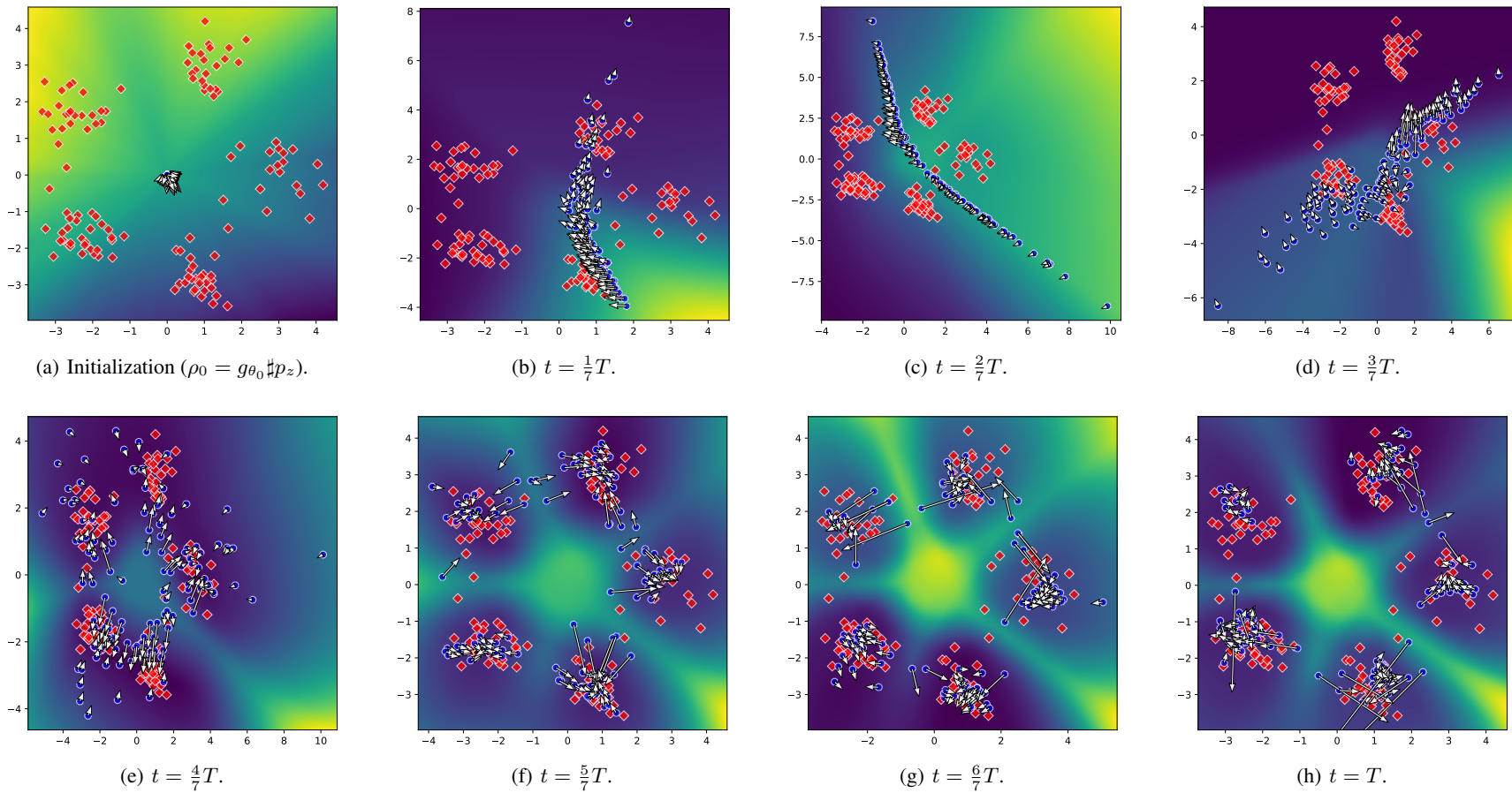
Figure 8: Training snapshots of a GAN on a Gaussian mixture; cf. Figure 6. Here time t represents training time, and T is the end of training. The colored backgrounds represent the pointwise generator loss function -h_{\rho_t} = -c \circ f_{\rho_t} (darker is lower, renormalized for every snapshot), from which the particle gradients, shown in the figures, are derived and then fed to the generator following Equations (11) and (13).
