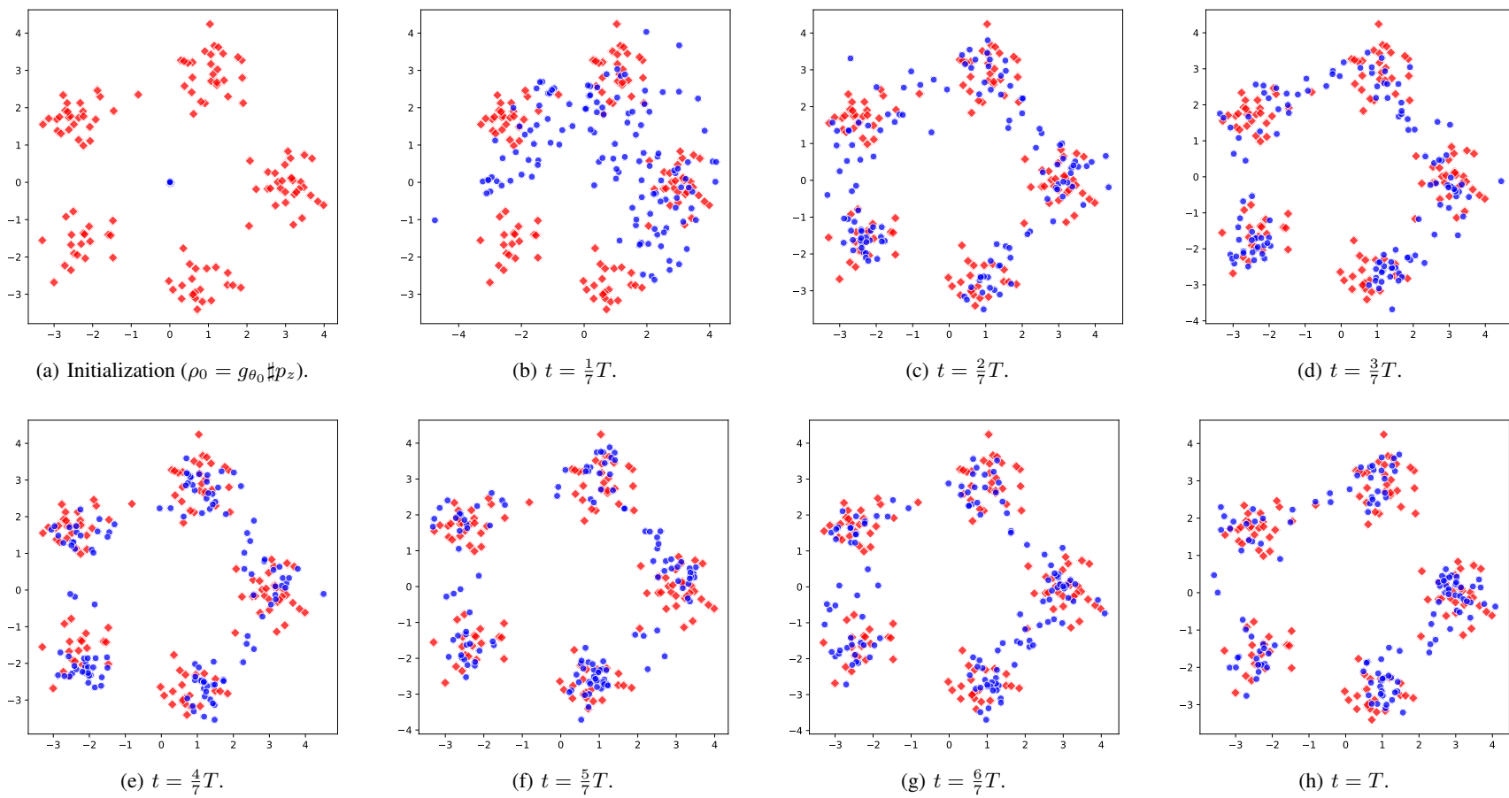
Figure 9: Training snapshots of a Score GAN on a Gaussian mixture; cf. Figure 6. Here time t represents training time, and T is the end of training.
