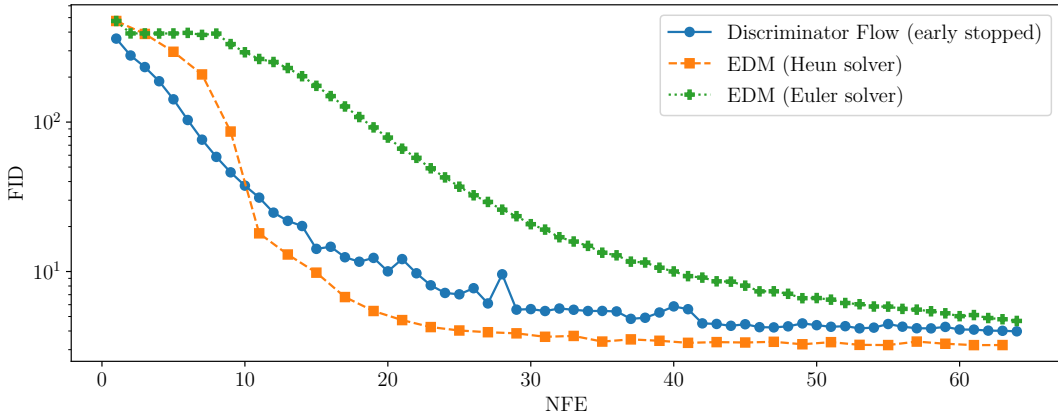
(b) Stopping the generative process of Equation (20) at an earlier time T' than in training ( 0 < T' < T = 1 ).
