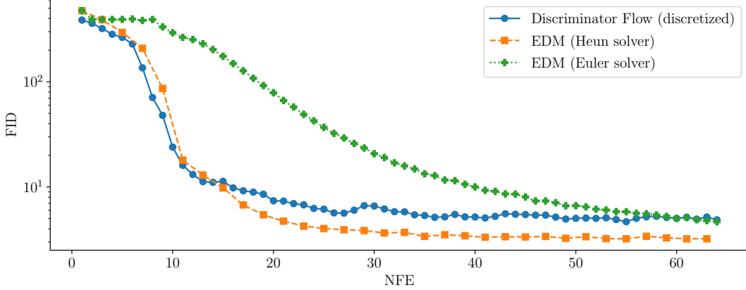
(a) Changing the differential equation time discretization of Equation (20) for Discriminator Flow.
