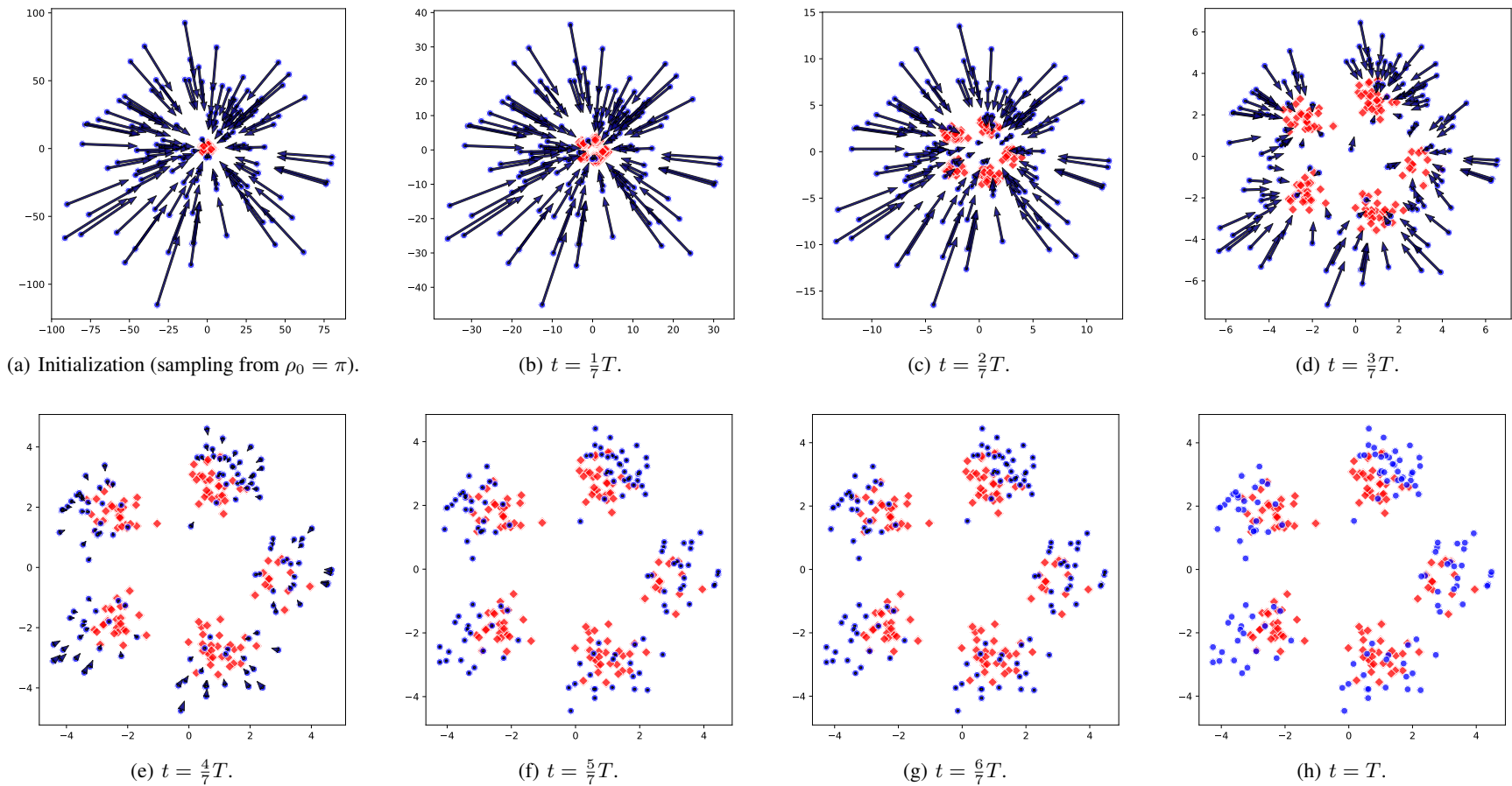
Figure 6: Sampling steps for EDM on a Gaussian mixture; 128 samples are shown for both the generated ( \bullet ) and the data ( \blacklozenge ) distributions. The second-order solver was used with 13 NFEs. Arrows show the gradients \nabla h_{\rho_t} associated with each generated sample, corresponding to the direction provided by the score function, cf. Equation (8).
