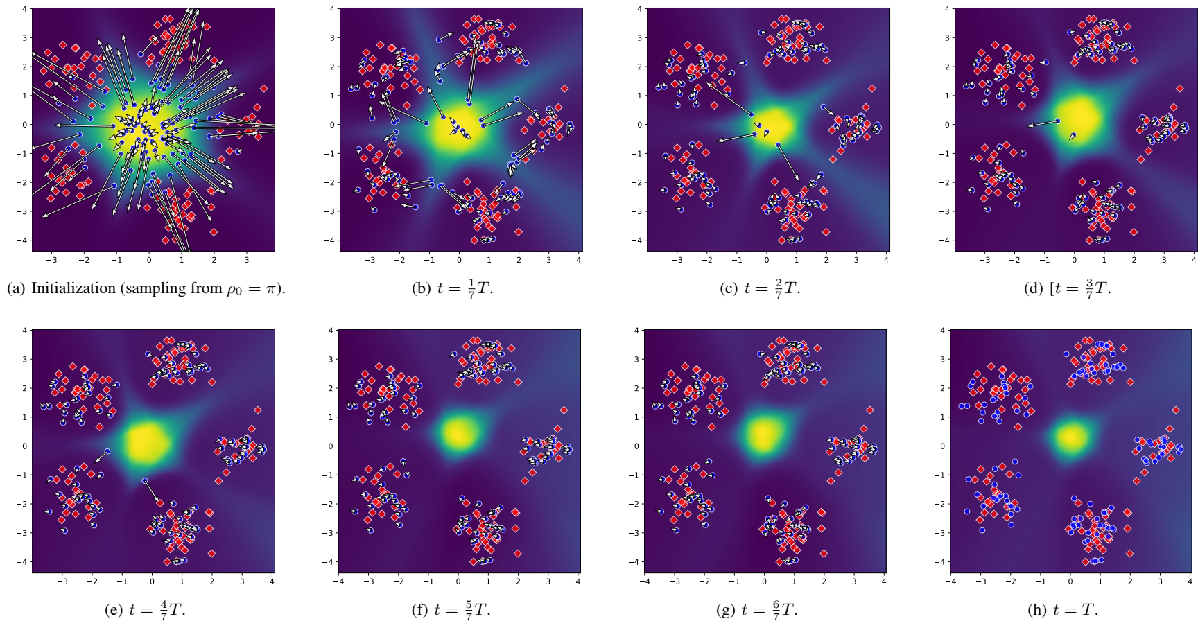
Figure 7: Sampling steps for Discriminator Flows on a Gaussian mixture; cf. Figure 6. Our chosen discretization yields 14 NFEs. The colored background represents the pointwise generator loss function -h_{\rho_t} = -c \circ f_{\rho_t} (darker is lower, renormalized for every snapshot), from which the particle gradients, shown in the figures, are derived.
