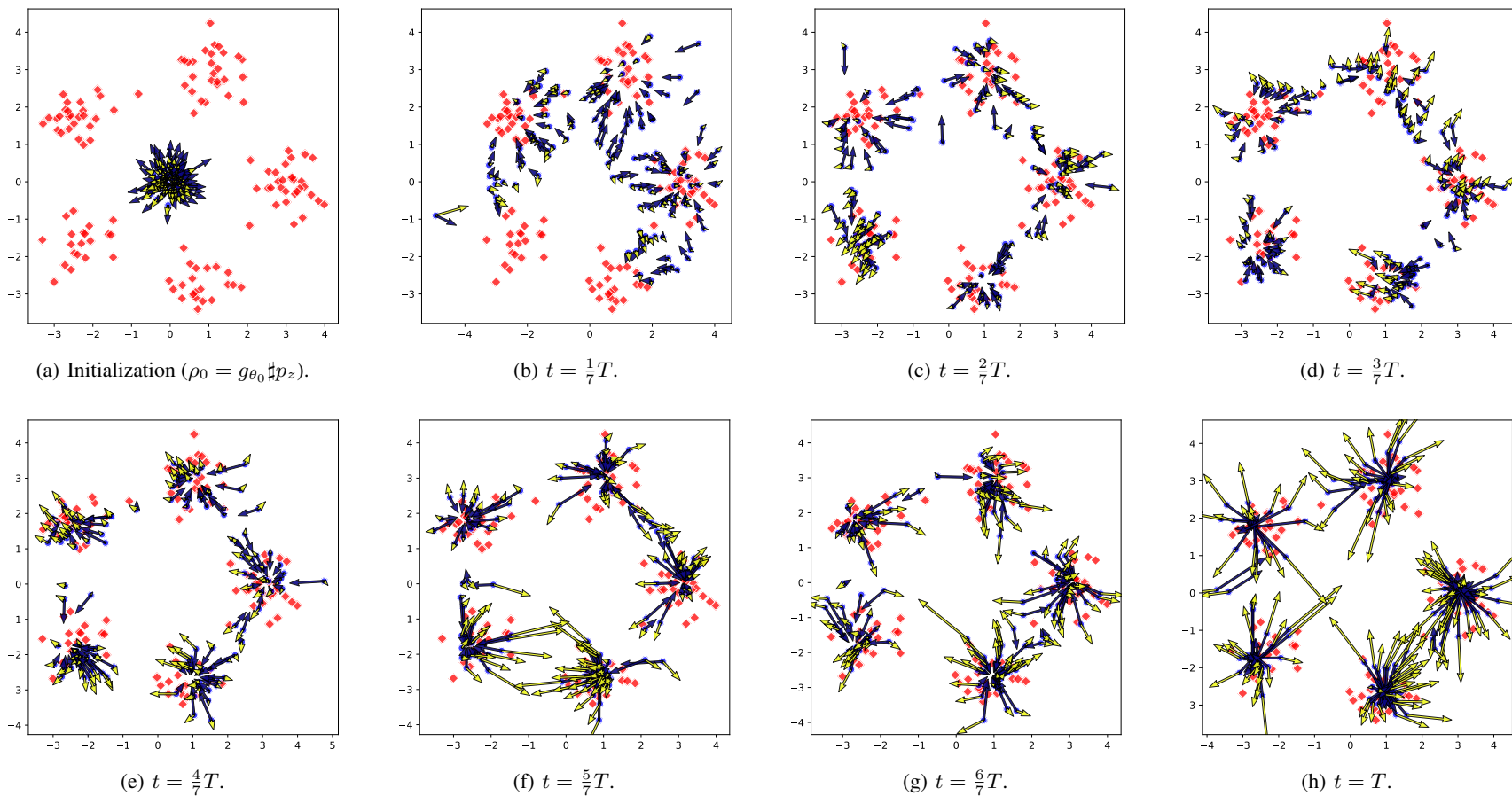
Figure 10: Training snapshots of a Score GAN on a Gaussian mixture identical to Figure 9, but with generated samples perturbed by Gaussian noise of standard deviation \sigma = 0.2 . Arrows show the gradients \nabla h_{\rho_t} received by the generated particles at this noise level, corresponding to Equation (19), split into the data score (in blue) and minus the score of the generated distribution (in yellow). They are then fed to the generator following Equations (11) and (13).
