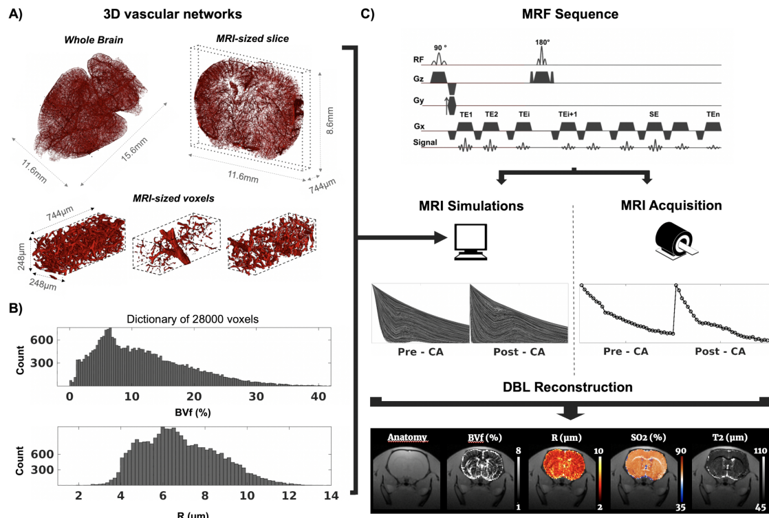
Figure 1: a) Top. Examples of the whole-brain vascular network and a single 744 \mu\text{m} thick slice from dataset 1. Both are eroded for visibility. Bottom. Three examples of MRI-sized voxels obtained. b) Distributions of BVf and mean radius in the 28,000 voxels generated. c) Overview of the MRF process: a sequence is used both for numerical simulations and for in-vivo acquisitions. Parametric maps are obtained either by comparing acquisitions to simulations (DBM), or by using Dictionary-based Learning (DBL).
