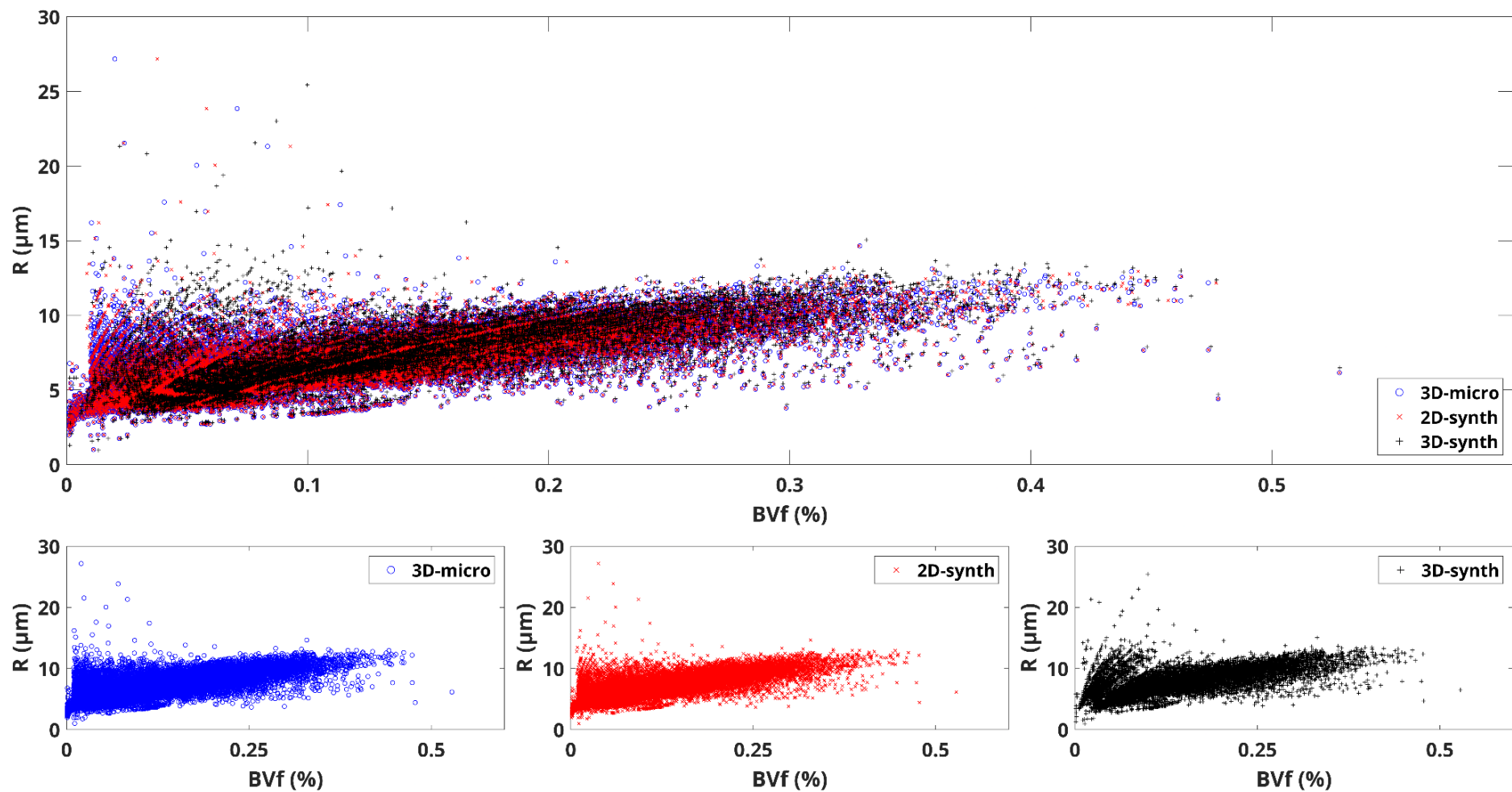
Sup. Fig. 2: (BVf, R) parameter space coverage for the three dictionaries generated. Top panel shows a superposition of the 3 lower panels, each corresponding to a dictionary. Discrepancies between the microscopy-based results and the synthetic ones come from the geometrical impossibility of our generation methods to accommodate every BVf and R combination.
