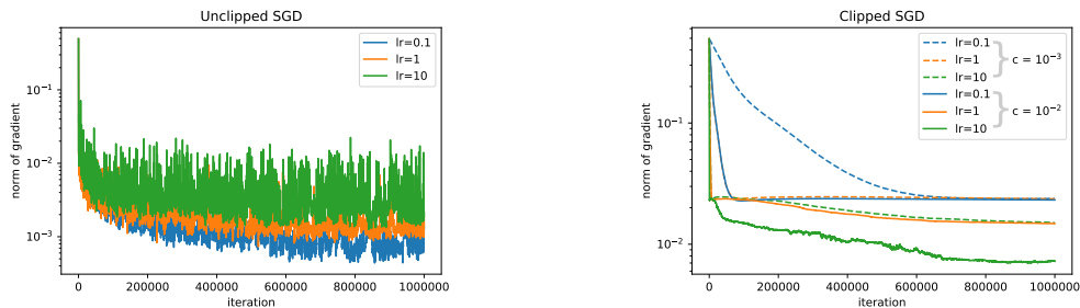
Figure 2. Stochastic gradient descent (with batch size = 1) on the w1a datasets. Without clipping, decreasing the stepsize allows to achieve smaller gradient norm (left). However, decreasing the stepsize with clipping does not allow to achieve better gradient norm, but even degrades its final norm (right). Similarly, increasing the clipping threshold c allows to reduce the final accuracy, as predicted by theory.
