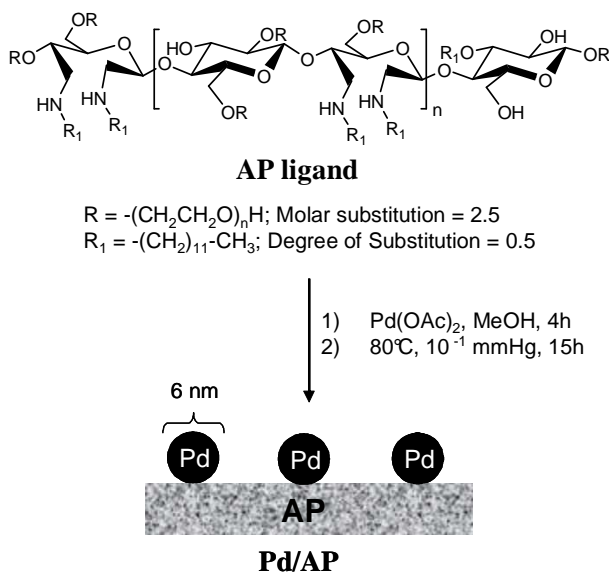
Scheme 2: Stabilization of Pd nanoparticles on AP
