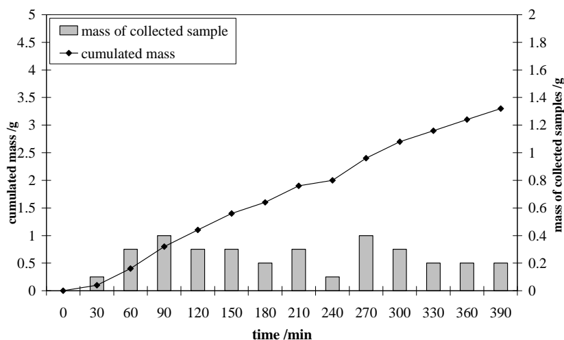
Figure 1: Extraction of the reaction products from glycerol using the scCO 2 technology.
