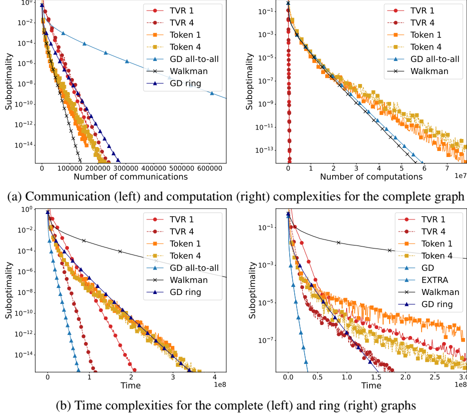
Figure 4: Convergence results for a logistic regression task on the RCV1 dataset [Lewis et al., 2004] ( d = 47236 ), with n = 20 nodes, and m = 9841 samples per node.
