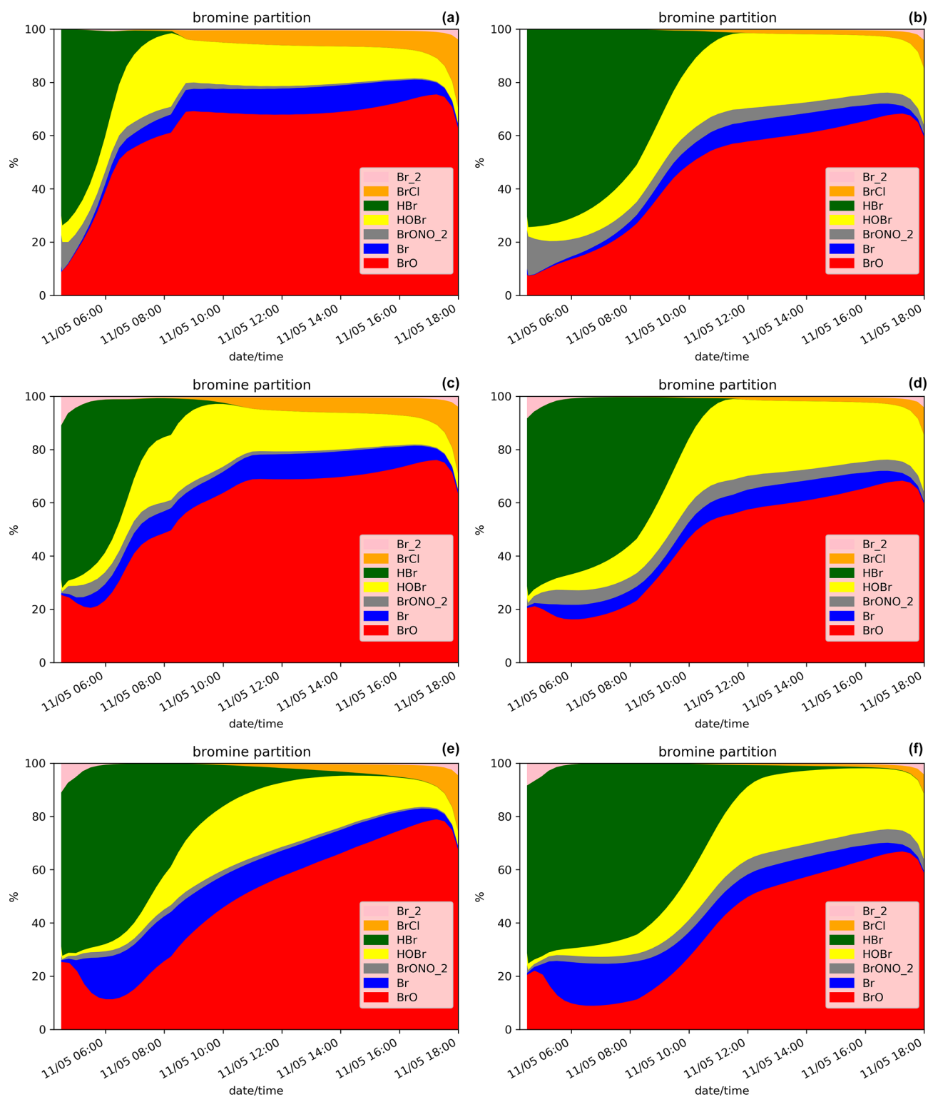
Figure 6. Similar to Fig. 5 but for the simulations D.LowHBr (a), D.Low.Emis (b), D.LowHBr.Plume.0.3 (c), D.Low.Emis.Plume.0.3 (d), D.LowHBr.Plume.0.1 (e) and D.Low.Emis.Plume.0.1 (f).
