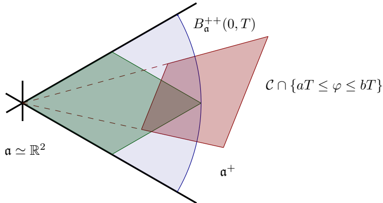
Figure 1: This is a positive Weyl chamber for \mathrm{SL}(3, \mathbb{R}) and T > 0 is large. In blue, our counting region B_{\mathfrak{a}^{++}}(0, T) . In green, Deitmar-Gon-Spilioti's [DGS19] counting region. In red, Guedes Bonthonneau-Guillarmou-Weich's [GBGW21] counting region where \mathcal{C} is a convex cone strictly inside \mathfrak{a}^{++} delimited by the red dashed lines, 0 < a < b are real numbers and \varphi is a linear form strictly positive on \mathfrak{a}^+ .
