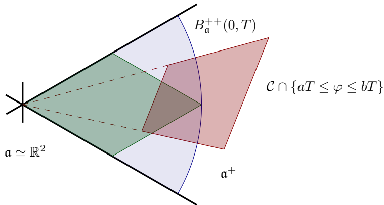
Figure 1: This is a positive Weyl chamber for \text{SL}(3, \mathbb{R}) and T > 0 is large. In blue, our counting region B_{\mathfrak{a}^{++}}(0, T) . In green, Deitmar-Gon-Spilioti's [DGS19] counting region. In red, Guedes Bonthonneau-Guillarmou-Weich's [GBGW21] counting region where \mathcal{C} is a convex cone strictly inside \mathfrak{a}^{++} delimited by the red dashed lines, 0 < a < b are real numbers and \varphi is a linear form strictly positive on \mathfrak{a}^+ .
