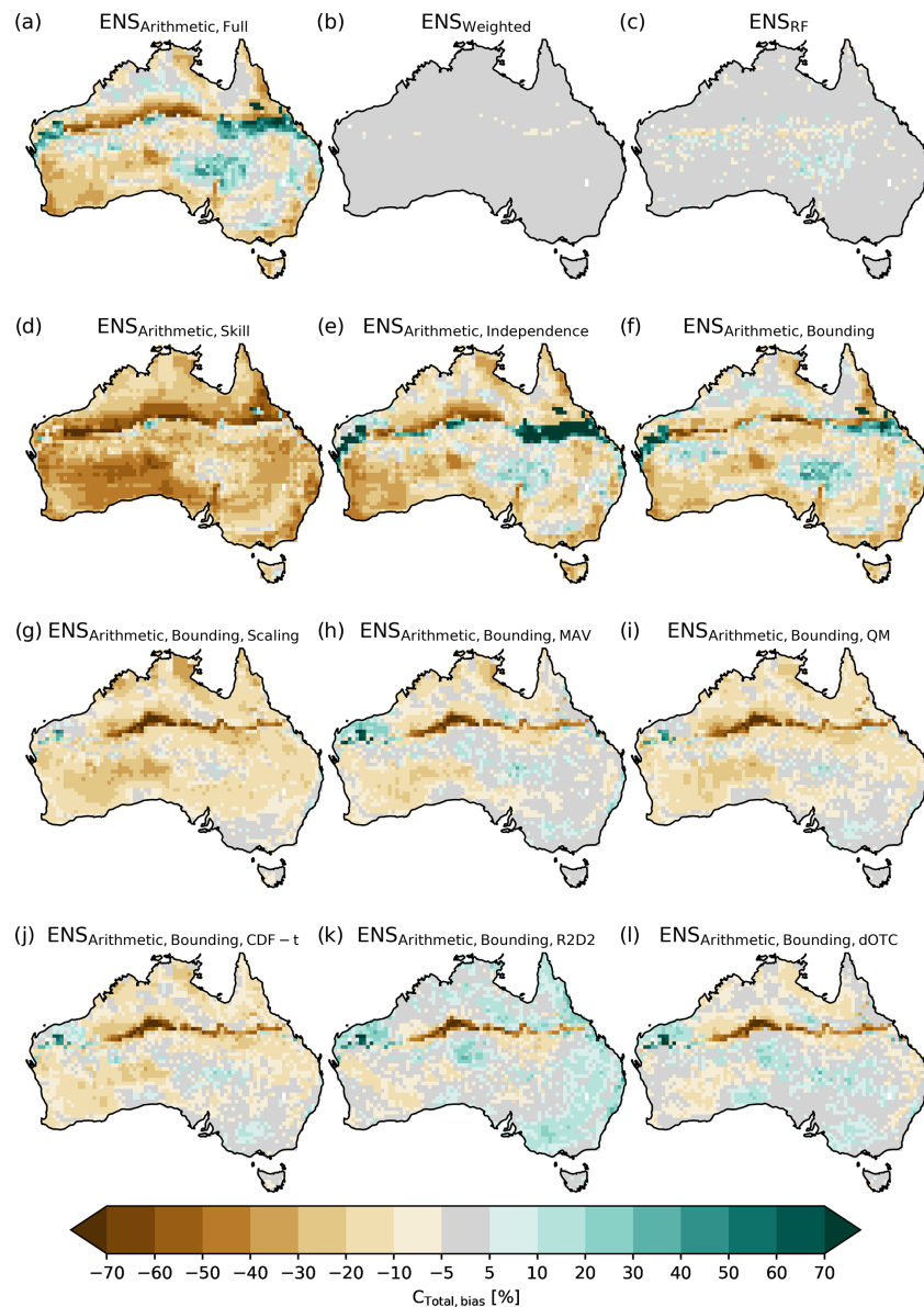
Figure 5. Difference between the ensemble averages of C_{\text{Total}} and C_{\text{Total}} simulated by \text{LG}_{\text{CRUJRA}} . Panels (a)–(c) show the arithmetic, weighted, and random forest ensemble average based on the LPJ-GUESS runs using the full CMIP6 ensemble, respectively. Panels (d)–(f) show the arithmetic ensemble average based on LPJ-GUESS runs using sub-selections of the CMIP6 ensemble (skilled, independent, and bounding GCMs, respectively). Panels (g)–(l) show the arithmetic ensemble average based on LPJ-GUESS runs using the bias-corrected bounding GCMs following the scaling, MAV, QM, CDF-t, R2D2, and dOTC approach, respectively. The noticeable bias across the Tropic of Capricorn results from the assumed bioclimatic limit for C_4 grasses.
