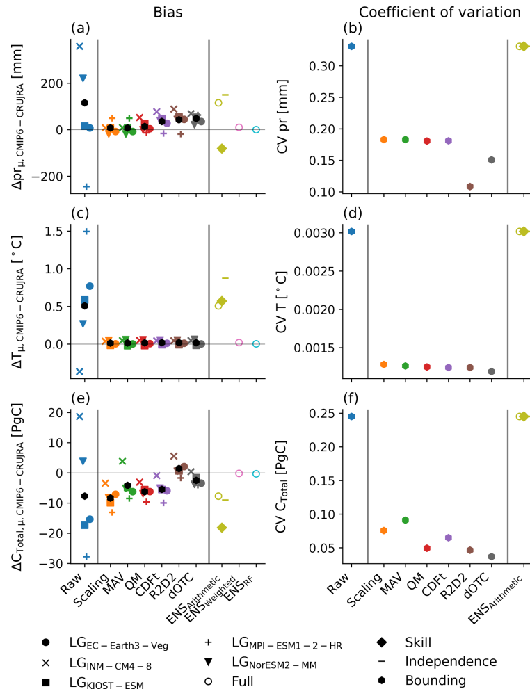
Figure 3. Difference between precipitation ( pr ), temperature ( T ), and carbon storage ( C_{\text{Total}} ) based on the CMIP6 and CRUJRA forcing (a, c, e) and the coefficient of variance across the ensemble of the same variables averaged over Australia. The different colors represent the results based on the raw (blue) or corrected climate forcing using scaling (orange), mean and variance (MAV, green), quantile mapping (QM, red), cumulative distribution function – transform (CDF-t, purple), dynamical optimal transport correction (dOTC, brown), and matrix re-correlation (R2D2, dark grey) approaches and the three ensemble-averaging methods (arithmetic mean (olive), weighted average (pink), and random forest (cyan)). The different symbols show LPJ-GUESS runs forced with the five bounding models, i.e., EC-Earth3-Veg (filled circle), INM-CM4-8 (x), KIOST-ESM (square), MPI-ESM1-2-HR (+), and NorESM2-MM (triangle), the full ensemble (empty circle), and the three model selection methods, i.e., skill (diamond), independence (horizontal bar), and bounding models (hexagon). The black hexagons depict the ensemble average of the LPJ-GUESS runs based on the raw and corrected bounding climate forcing.
