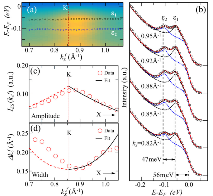
FIG. 6. (a) Close-up of 6H ZZ-sidewall ribbon band structure near E_F [dashed box in Fig. 5(a)] showing flat bands, \epsilon_1 and \epsilon_2 . Circles \circ mark the peak positions from EDC fits. (b) Sample EDCs near E_F in (a) ( \circ are data). A two-Lorentzian (dashed black and blue lines) plus background and Fermi-Dirac cutoff fit is shown (red solid line). Panels (c) and (d) show \epsilon_1 and \epsilon_2 average intensity and \Delta k_y^f width, respectively, vs k_x^f . Solid and dashed lines are TB estimates described in the text.
