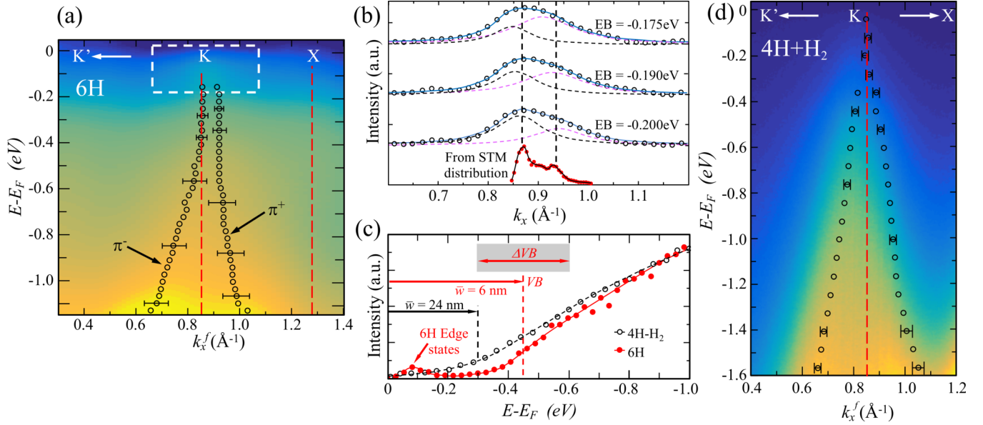
FIG. 5. (a) ARPES-measured bands of 6H ZZ-sidewall ribbons along the K'KT' direction (parallel to the ZZ edge). T_{\text{sample}} = 100 K. k_x^f is in the plane of the (11\bar{2} \sim 22) facet. Circles ( \circ ) mark the band positions. (b) Typical MDC fits showing the \pi -band asymmetry for BE > -0.4 eV. Solid red circles show the predicted asymmetry from the measured facet N(w_f) distribution and Eq. (1). (c) Integrated \pi -band intensity for 6H (red circles) and H_2 -passivated 4H ribbons (black circles). Red arrows mark the estimated valence band edge and width from 6H STM ribbon N(w_f) . (d) ARPES bands from H_2 -passivated 4H ZZ ribbons along the K'KX direction (30 nm steps). k_x^f is in the (11\bar{2} \sim 15)_{4H} plane.
