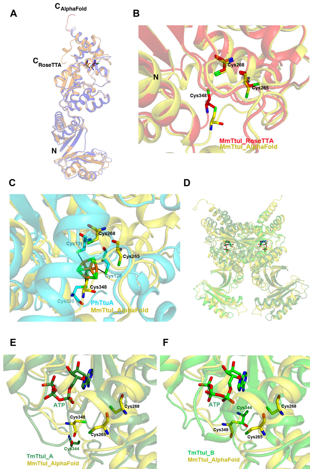
Figure 3. Best models of MmTtuI. (A) Superposition of the AlphaFold model, colored according to the pLDDT values, from red (pLDDT value of 37.0) to blue (pLDDT value of 98.8) and RoseTTAFold (in orange) model of the monomer of MmTtuI. (B) Superposition of the conserved cysteines of MmTtuI in the AlphaFold model (in yellow) and RoseTTAFold model (in red). The pLDDT values of Cys265, Cys268 and Cys348 in the AlphaFold model are 95.8, 95.9 and 89.4, respectively. (C) Superposition of the active sites of the MmTtuI AlphaFold model and holo-PhTtuA crystal structure (PDB code 5MKP, in cyan). Holo-PhTtuA was superimposed onto the MmTtuI model with the SUPER option in PYMOL, with an rmsd of 3.4 Å for 98 aligned C \alpha atoms. The cluster in holo-PhTtuA is shown in stick representation. (D) Superposition of the dimer of MmTtuI calculated with AlphaFold with that of the crystal structure of TmTtuI (in green and forest green for each monomer). ATP bound to TmTtuI is shown in stick representation. (E, F) Superposition of the active sites of the MmTtuI AlphaFold model and TmTtuI crystal structure (E: molecule A of TmTtuI; F, molecule B of TmTtuI). The MmTtuI model is superimposed on molecules A and B of the TmTtuI crystal structures with an rmsd of 1.37 Å for 281 aligned C \alpha atoms and an rmsd of 1.48 Å for 285 aligned C \alpha atoms, respectively. ATP and Cys344 in the TmTtuI structure are shown in stick representation.
