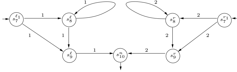
Figure 8: Path Automata Recognizing the Paths to Component Atoms from Example 6
