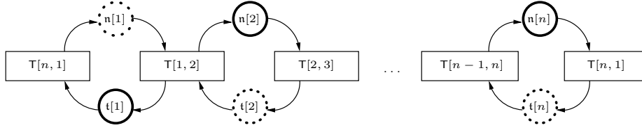
Figure 3: The Execution Semantics of a Token-Ring System
