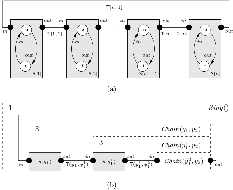
Figure 1: Recursive Specification of a Token-Ring System
