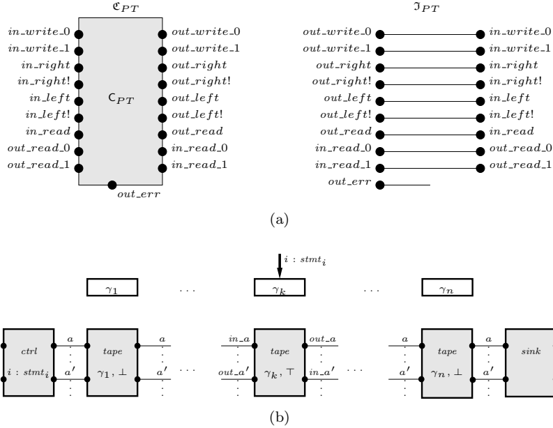
Figure 4: Undecidability of Deadlock and Reachability for Linear Component-based Systems
