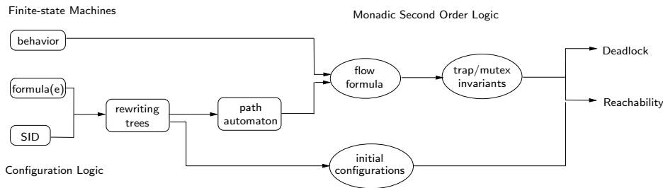
Figure 2: The Synthesis of Verification Conditions
