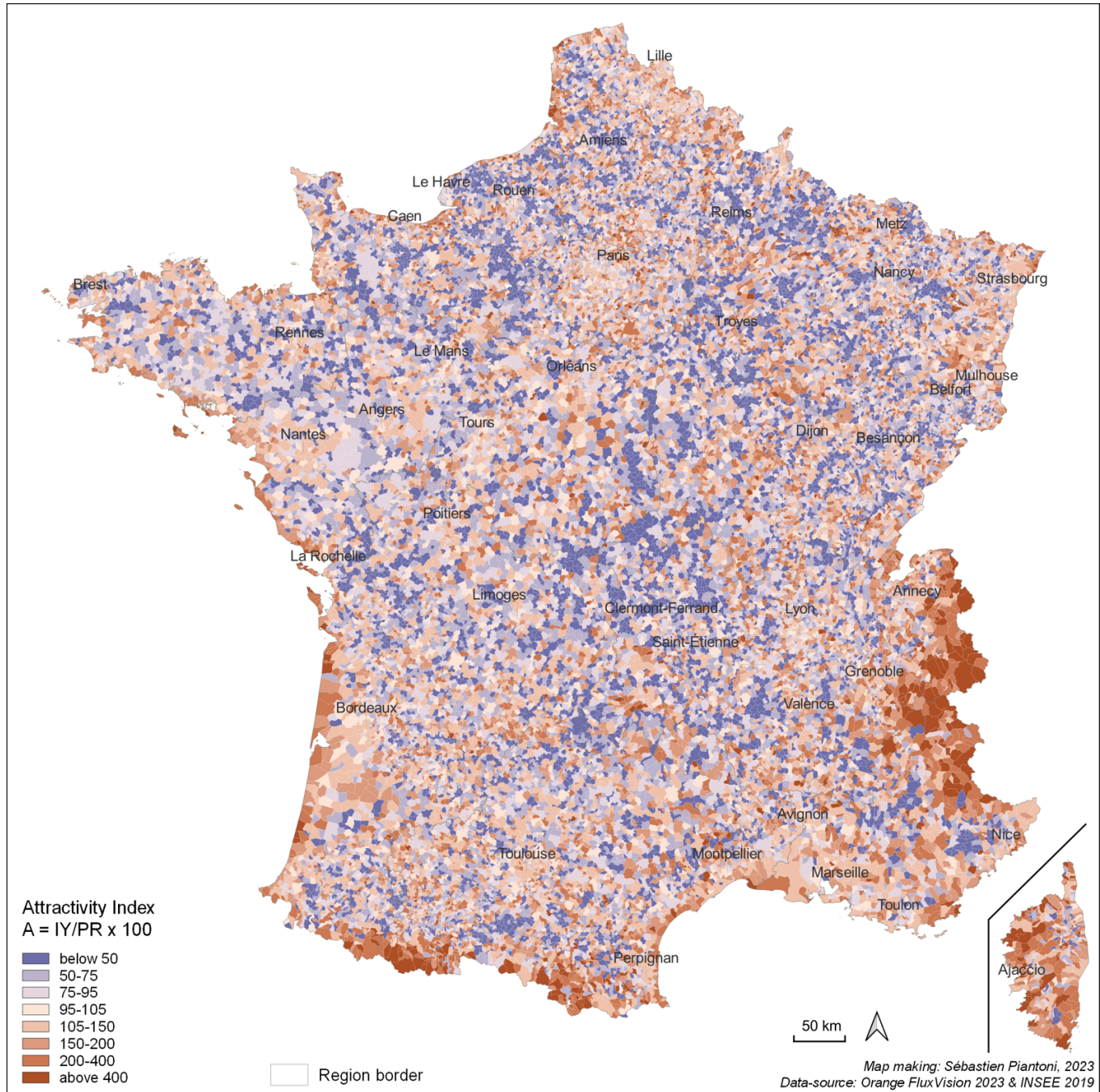
32 Fig. 3. France, A-index, Euclidean Metric. 33 34
