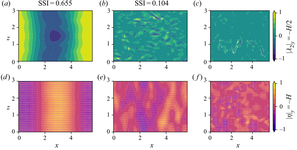
FIGURE 17. Slices of the normalised \lambda_2 criterion and interface displacement \eta , as observed during K-type (a,d, t = 100 ), F-type transition (b,e, t = 35 ) and for a fully developed turbulent state (c,f, t = 500 ). The values of the structural similarity index (SSI) (Wang et al. 2004) computed for the two panels of each column are reported on top of the columns.
