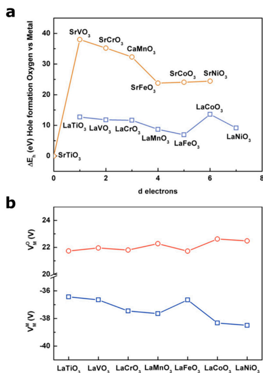
Figure 2. (a) Variation of the energy of hole formation on oxygen vs. hole formation on metal calculated from Equation (1) as a function of d electrons for cubic or pseudocubic LaM 3+ O 3 (blue) and AM 4+ O 3 (brown) perovskites. Note that 0 eV is arbitrarily given to SrTiO 3 ( d^0 ) as a reference. Madelung constants were obtained from Vesta software using reported structures, and the Madelung potentials were calculated from the method describe elsewhere [24]. The ionization energies were obtained from elsewhere [33]. CaMnO 3 was chosen due to its pseudocubic symmetry rather than SrMnO 3 which possesses hexagonal structure. Note that no Ni 4+ containing perovskite shows a pseudocubic lattice and SrNiO 3 used in this plot shows the hexagonal 2H structure. (b) Oxygen Madelung potentials ( V_M^O ) and metal Madelung potentials ( V_M^M ) calculated for the LaM 3+ O 3 series using a classical approach.
