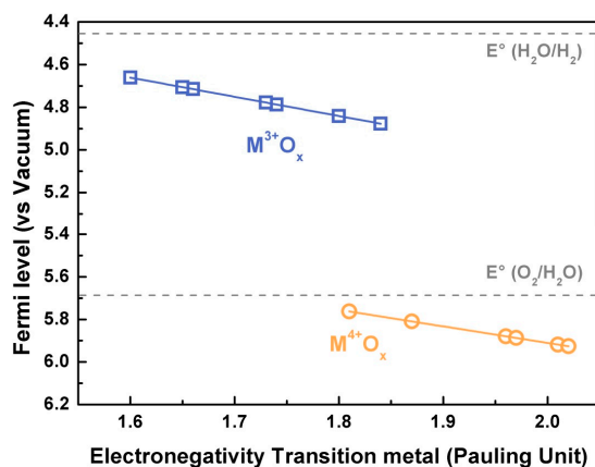
Figure 3. Fermi level calculated for M 3+ and M 4+ 3d metal following the simple equation developed by Campet et al. [28] as a function of the transition metal electronegativity (in Pauling unit) as calculated by Matar et al. [29]. The Fermi levels calculated with equation (2) correspond to the middle of the band gap, and are compared to the standard potential H 2 O/H 2 and O 2 /H 2 O at pH = 0.
