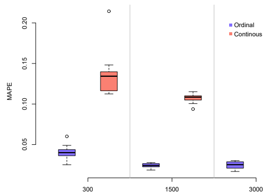
(c) MAPE for \Sigma
