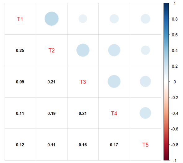
(b) Cluster 2
