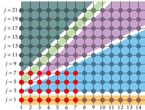
Fig. 20. The points on which the ratio conjecture is tested for 1 \leq c \leq 7 by the snippet "9. ratio" are shown in red.
