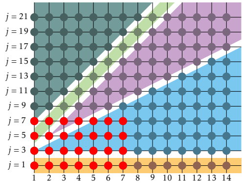
Fig. 18. The points on which the ratio conjecture is tested for 1 \leq c \leq 7 by the snippet "9. ratio" are shown in red.
