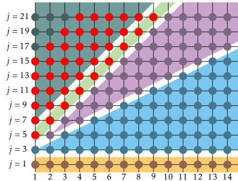
Fig. 19. The points on which Croatia is tested. Note that the test is performed directly at the (\alpha_{j,\kappa}, \beta_{j,\kappa}) -level. Points tested by the snippet "7. Croatia" are shown in red. Points tested beyond the quadrant are not shown.
