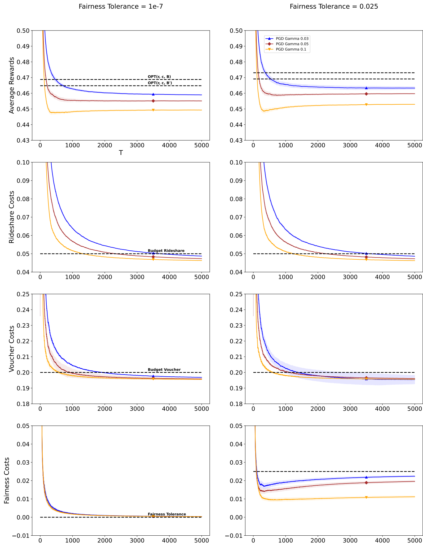
Figure 1: Performance of the PGD strategies.
